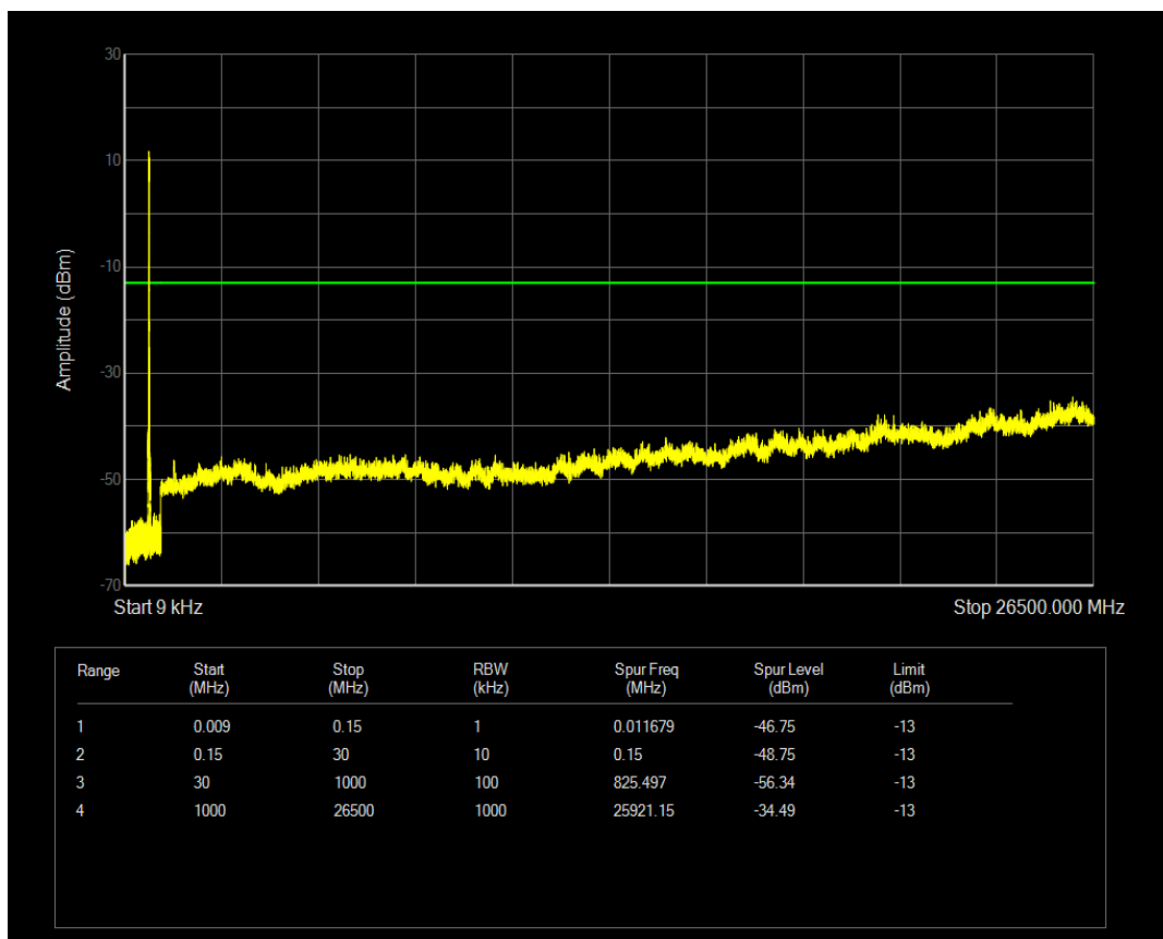
Band71 QAM16 BW=15MHz Channel=133297 RB Size=75 Position=#0
