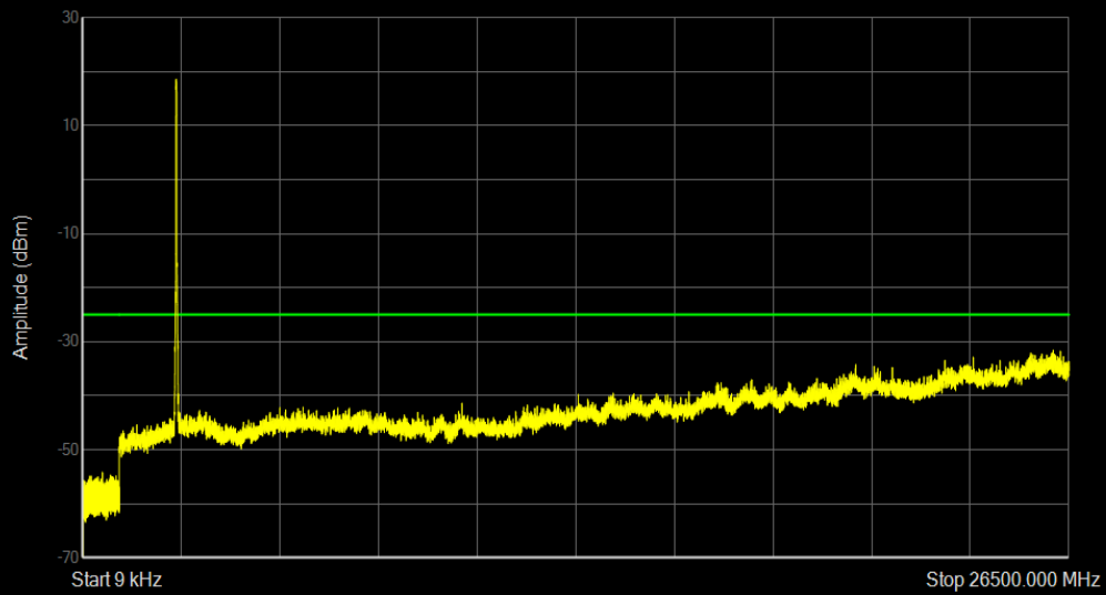
Band7 QAM16 BW=20MHz Channel=21100 RB Size=100 Position=#0
