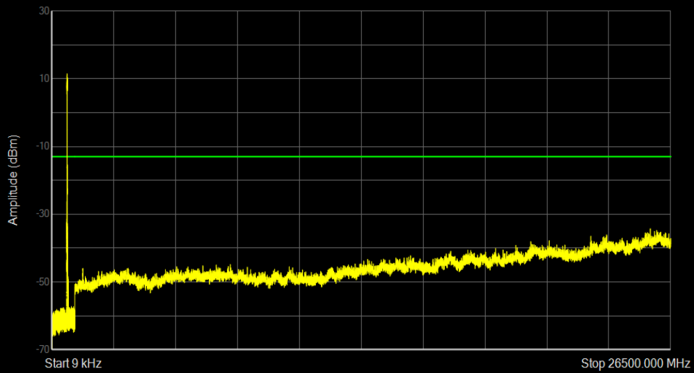
Band71 QPSK BW=15MHz Channel=133197 RB Size=75 Position=#0
