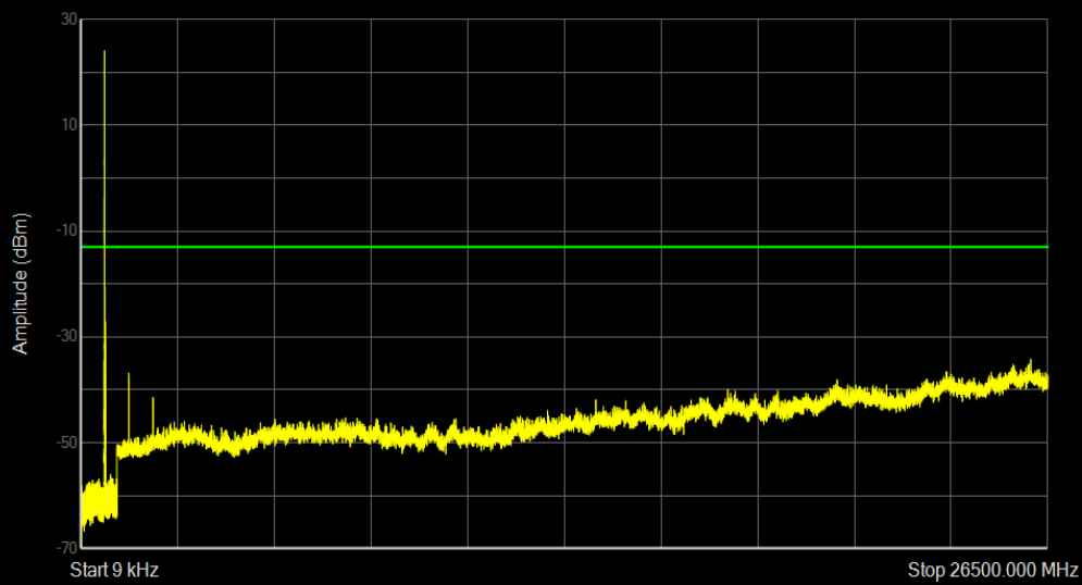
Band71 QPSK BW=10MHz Channel=133172 RB Size=1 Position=#0
