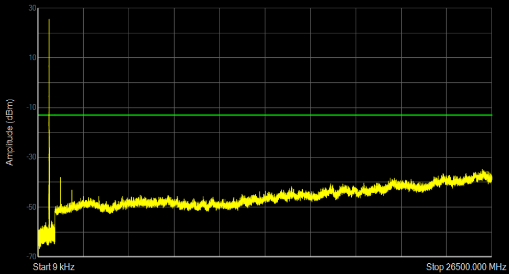
Band71 QAM16 BW=15MHz Channel=133197 RB Size=1 Position=#0
