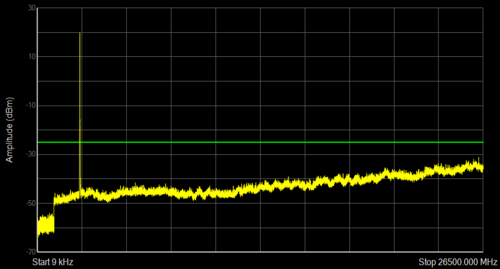
Band41 QPSK BW=10MHz Channel=40090 RB Size=50 Position=#0
