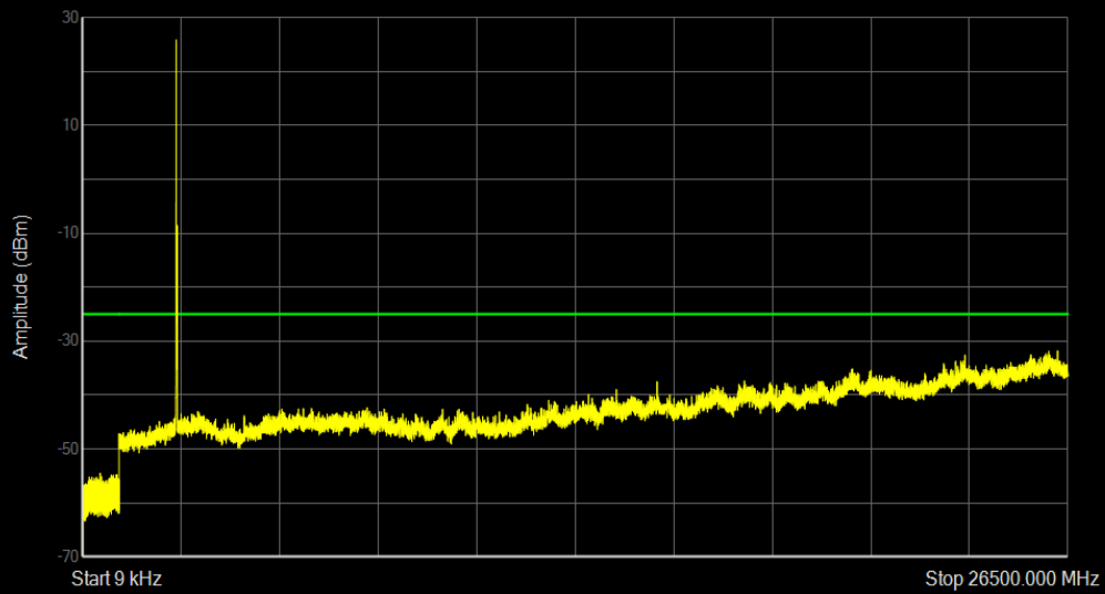
Band41 QPSK BW=15MHz Channel=40115 RB Size=1 Position=#0
