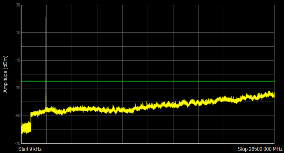
Band41 QAM16 BW=5MHz Channel=40640 RB Size=25 Position=#0
