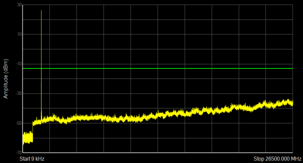
Band25 QPSK BW=1.4MHz Channel=26047 RB Size=6 Position=#0
