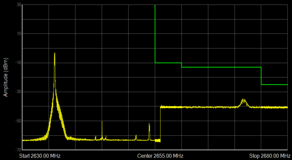
Band41 QAM16 BW=20MHz Channel=41140 RB Size=1 Position=#0
