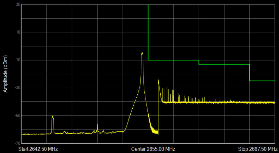
Band41 QPSK BW=10MHz Channel=41190 RB Size=1 Position=#Max
