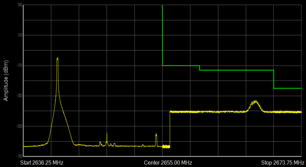
Band41 QPSK BW=15MHz Channel=41165 RB Size=1 Position=#0
