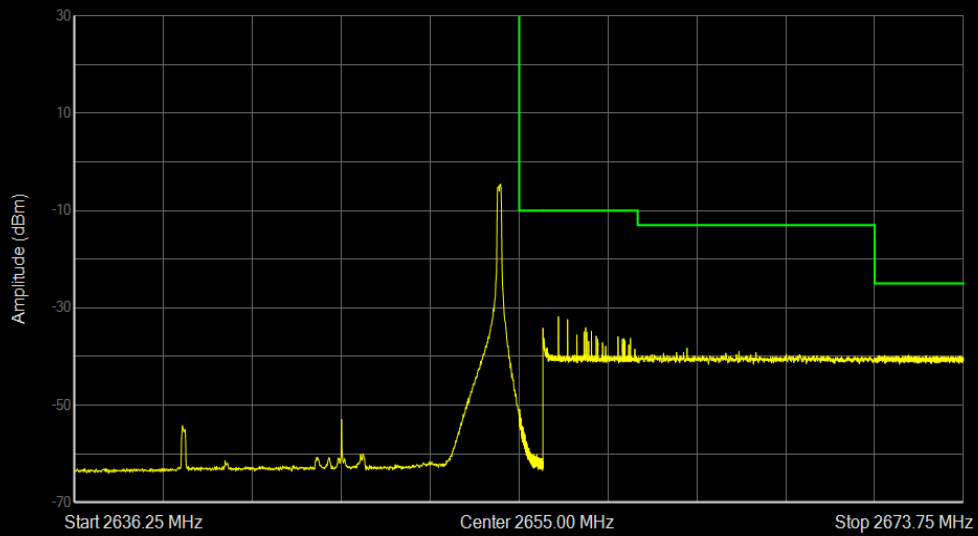
Band41 QPSK BW=15MHz Channel=41165 RB Size=1 Position=#Max
