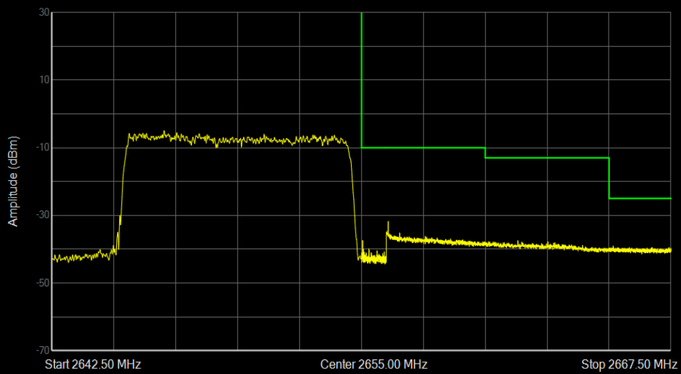
Band41 QPSK BW=10MHz Channel=41190 RB Size=50 Position=#0
