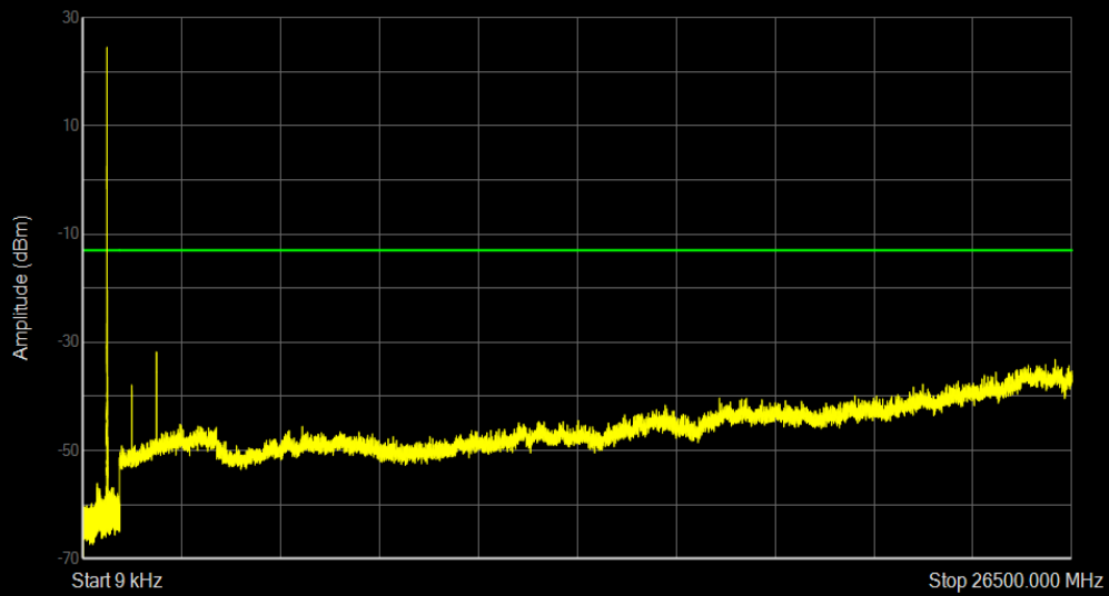
Band71 QAM16 BW=5MHz Channel=133147 RB Size=1 Position=#0
