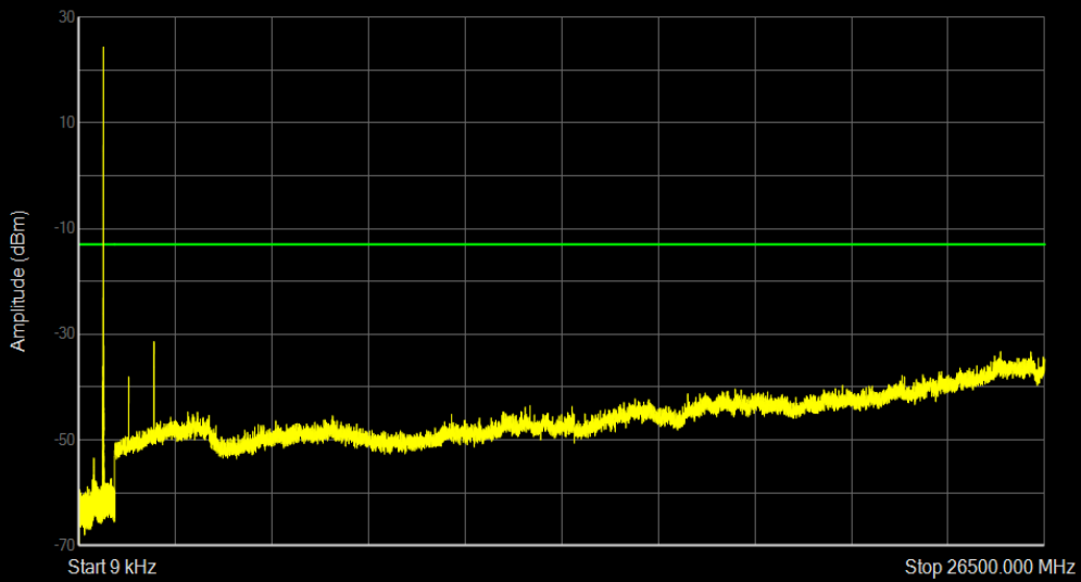
Band71 QPSK BW=5MHz Channel=133447 RB Size=1 Position=#0
