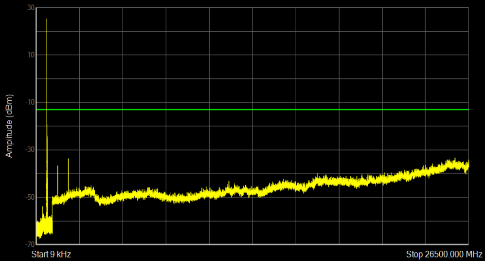
Band71 QPSK BW=10MHz Channel=133172 RB Size=1 Position=#0
