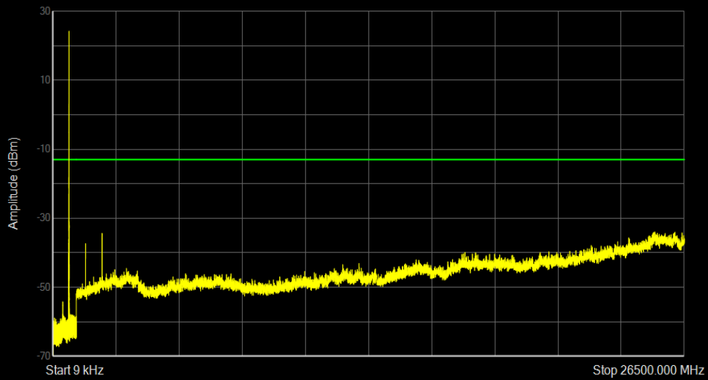
Band71 QAM16 BW=5MHz Channel=133447 RB Size=1 Position=#0
