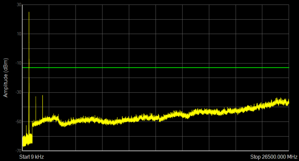
Band71 QAM16 BW=10MHz Channel=133297 RB Size=1 Position=#0
