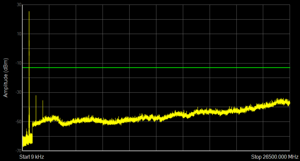
Band71 QAM16 BW=20MHz Channel=133372 RB Size=1 Position=#0
