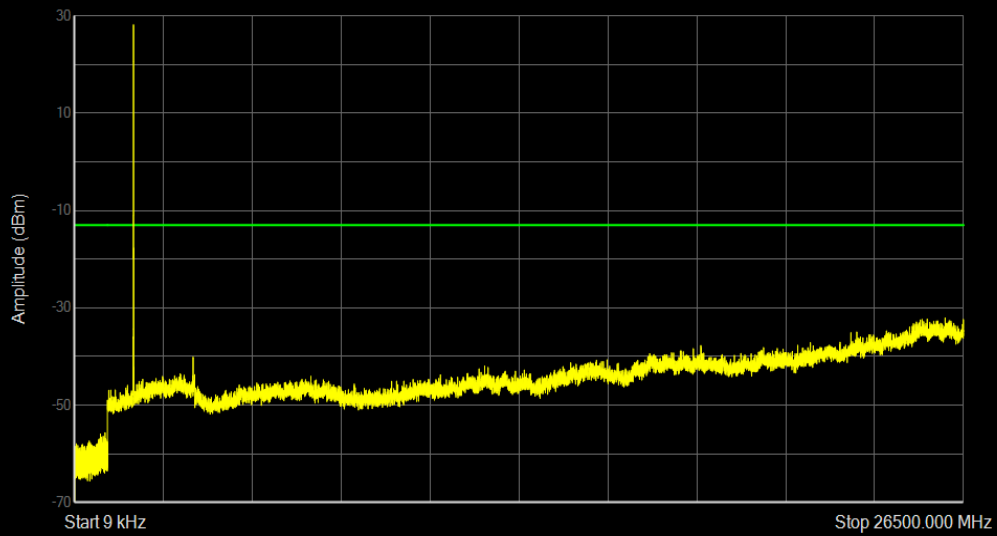
Band66 QAM16 BW=5MHz Channel=132647 RB Size=1 Position=#0
