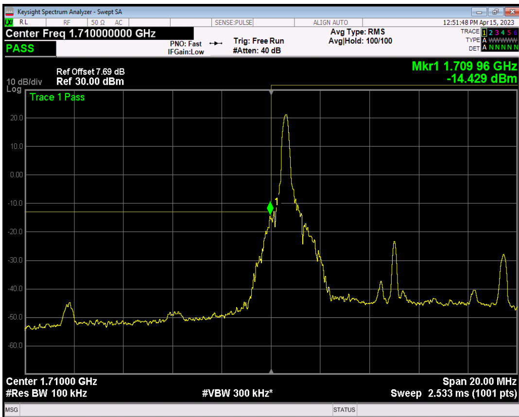
Band66 QAM16 BW=10MHz Channel=132022 RB Size=1 Position=#Max
