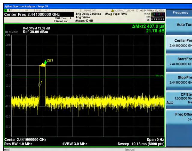
3DH3-Ant1-Hop-1.657-160
