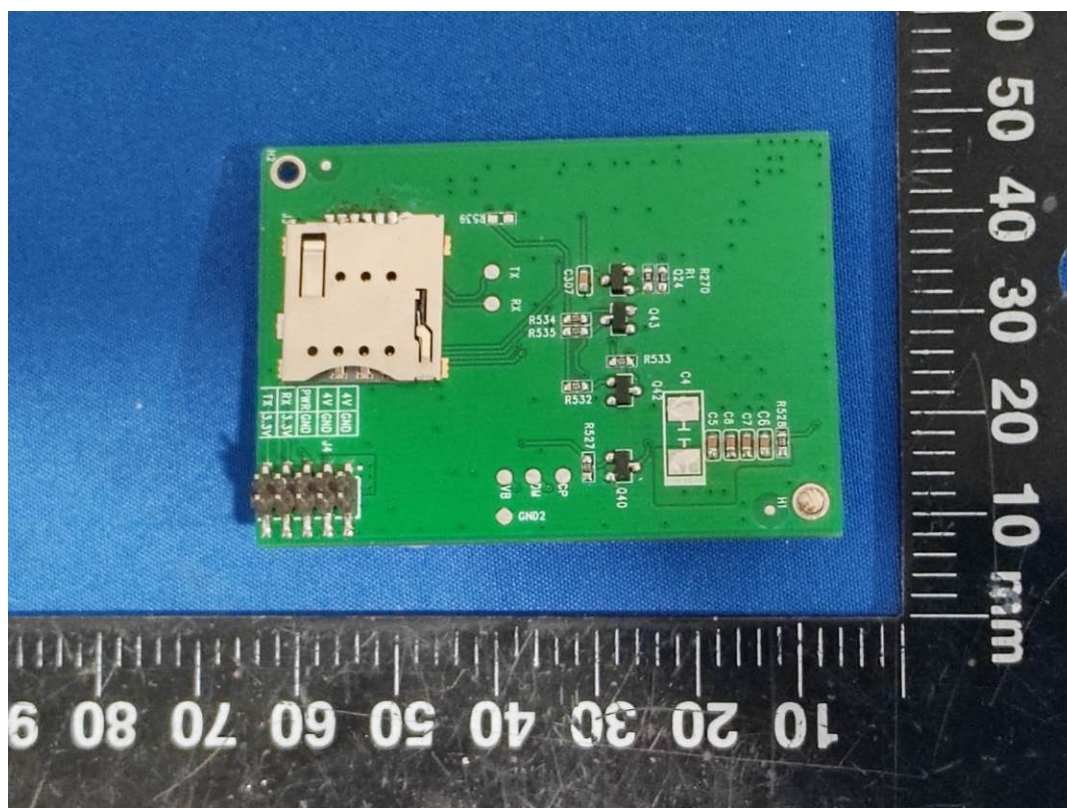
WWAN Module: EC25-AFXD, FCC ID: XMR202008EC25AFXD, IC:10224A-022EC25AFXD
