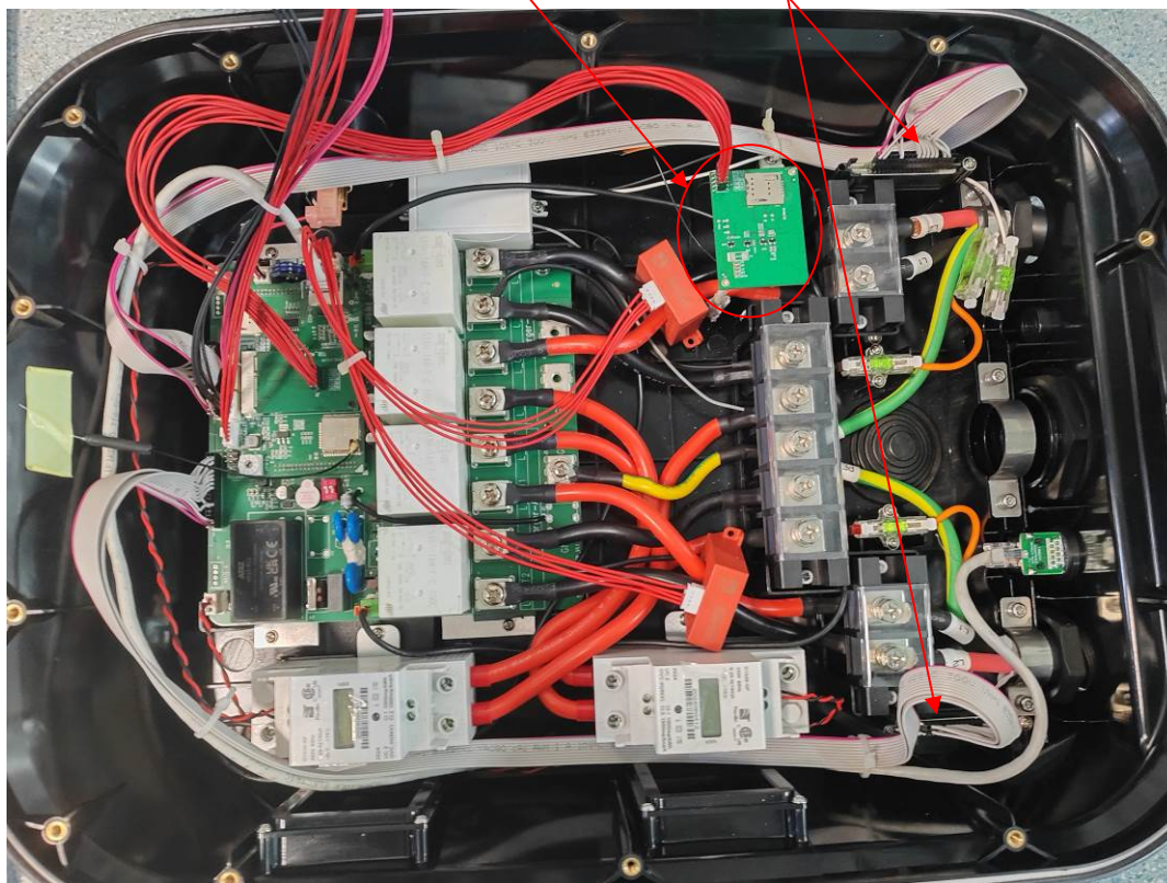
WWAN Module Location
