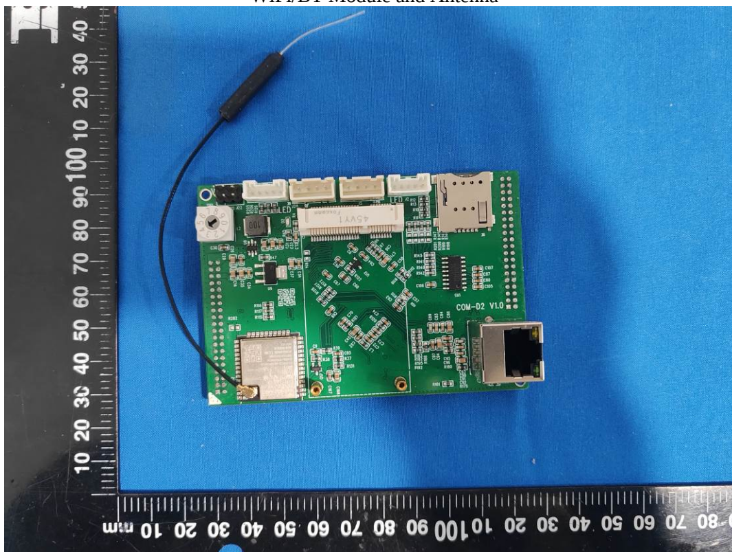
WiFi/BT Module: ESP32-WROOM-32U, FCC ID: 2AC7Z-ESP32WROOM32U, IC:21098-ESP32WROOM32U
