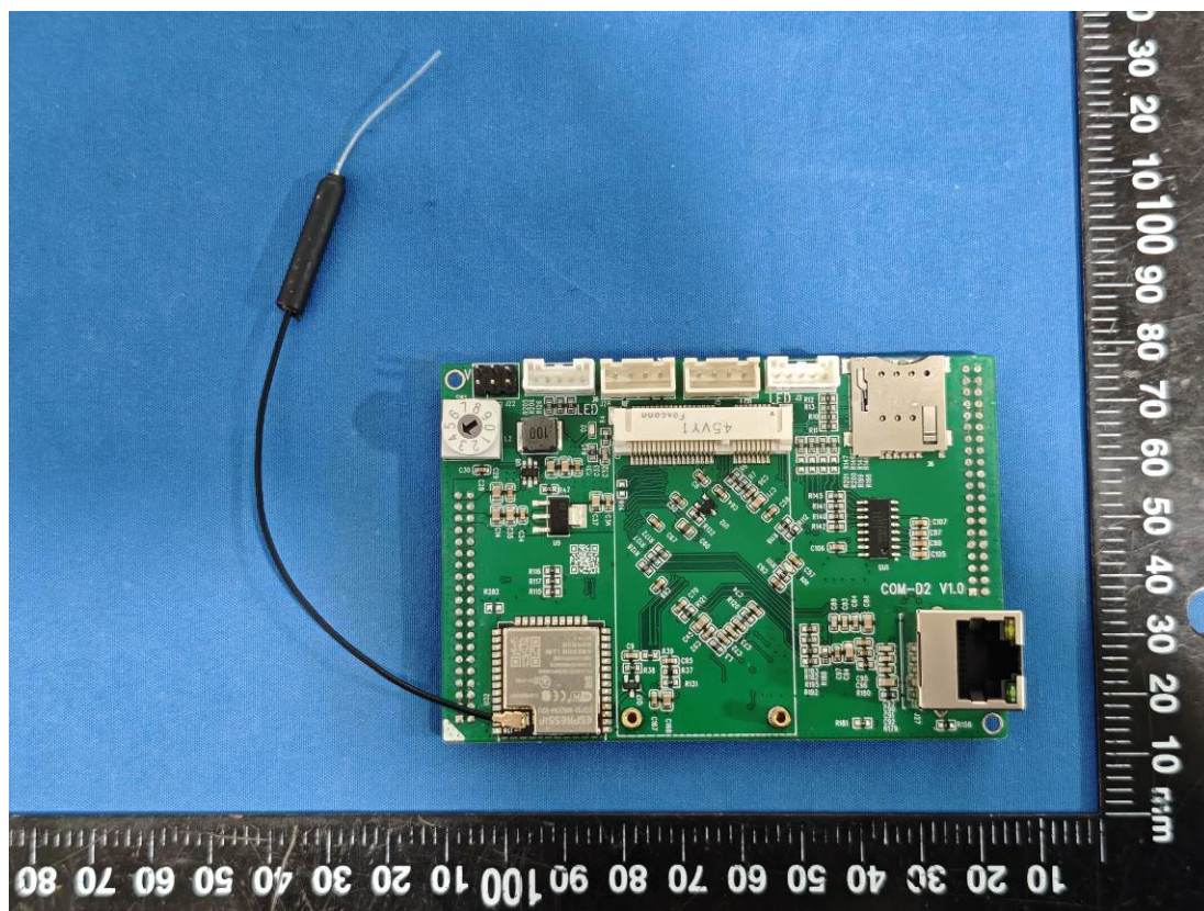
WiFi/BT Module and Antenna
