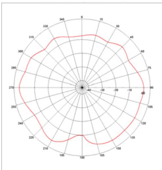
Far-field Power Distribution(H+V) on Y-Z Plane
