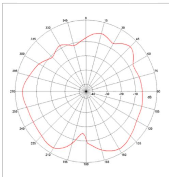
Far-field Power Distribution(H+V) on X-Z Plane
