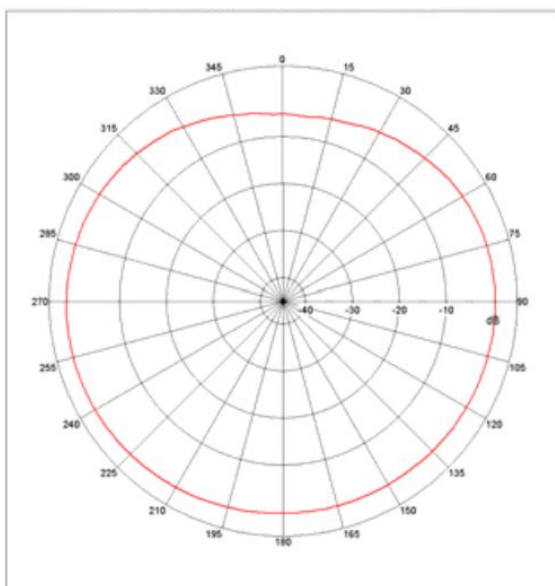
Far-field Power Distribution(H+V) on X-Y Plane
