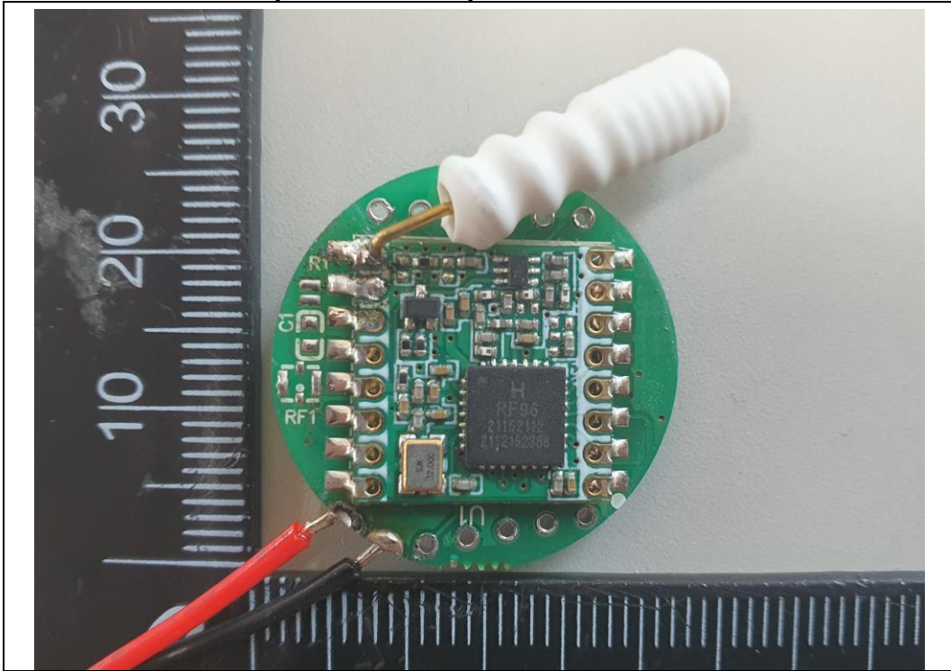
Main Board_Front (COWSEN-003)
