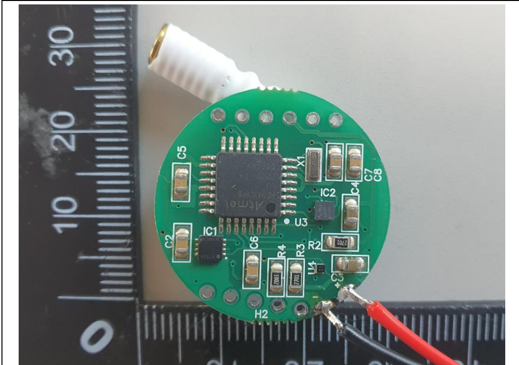
Main Board_Rear (COWSEN-003)
