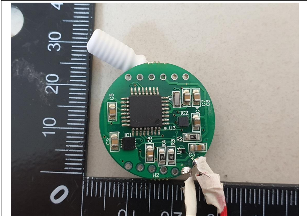
Main Board_Rear (COWTAG)
