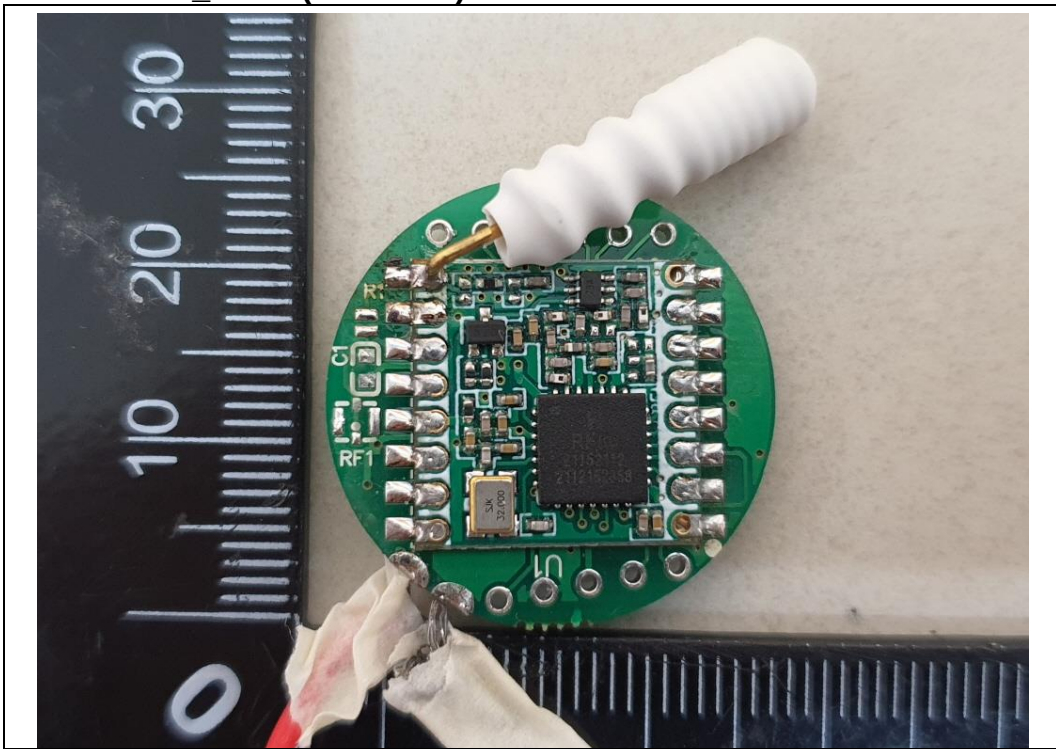
Main Board_Front (COWTAG)
