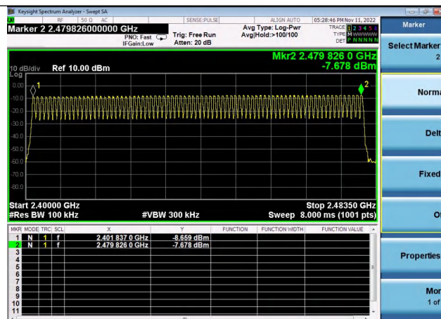
GFSK Modulation
