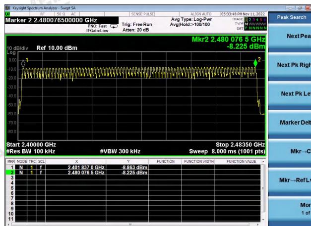
8-DPSK Modulation
