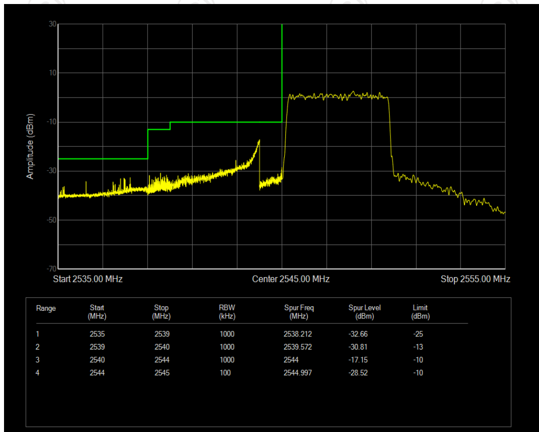
Band41(2545-2655) QPSK BW=5MHz Channel=40165 RB Size=25 Position=#0
