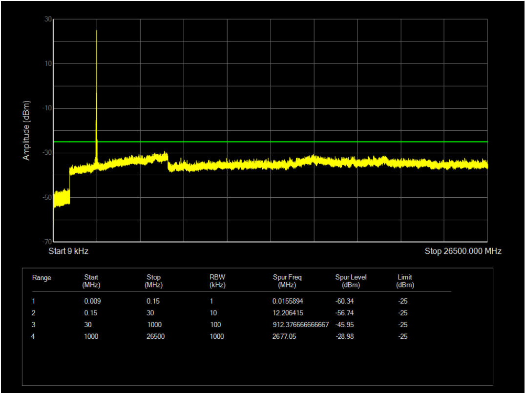
Band41(2545-2655) QPSK BW=10MHz Channel=40190 RB Size=1 Position=#0
