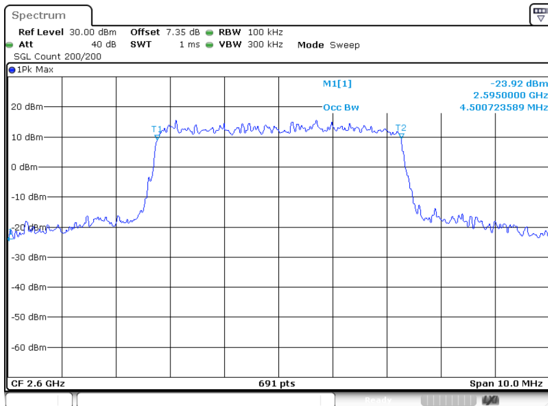
Band41(2545-2655) QPSK BW=5MHz Channel=40690 RB Size=25 Position=#0
