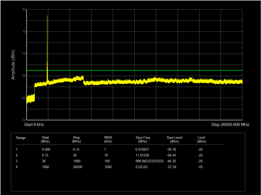
Band41(2545-2655) QPSK BW=5MHz Channel=41215 RB Size=1 Position=#0
