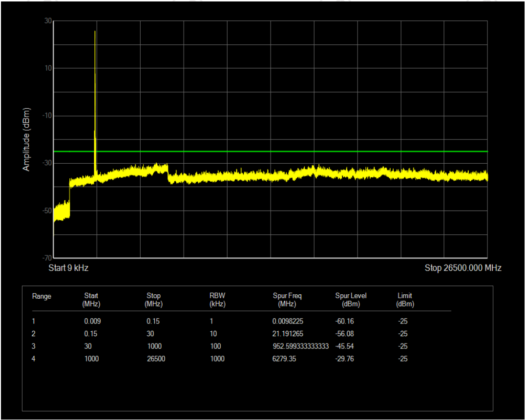
Band41(2545-2655) 16QAM BW=10MHz Channel=40190 RB Size=1 Position=#0
