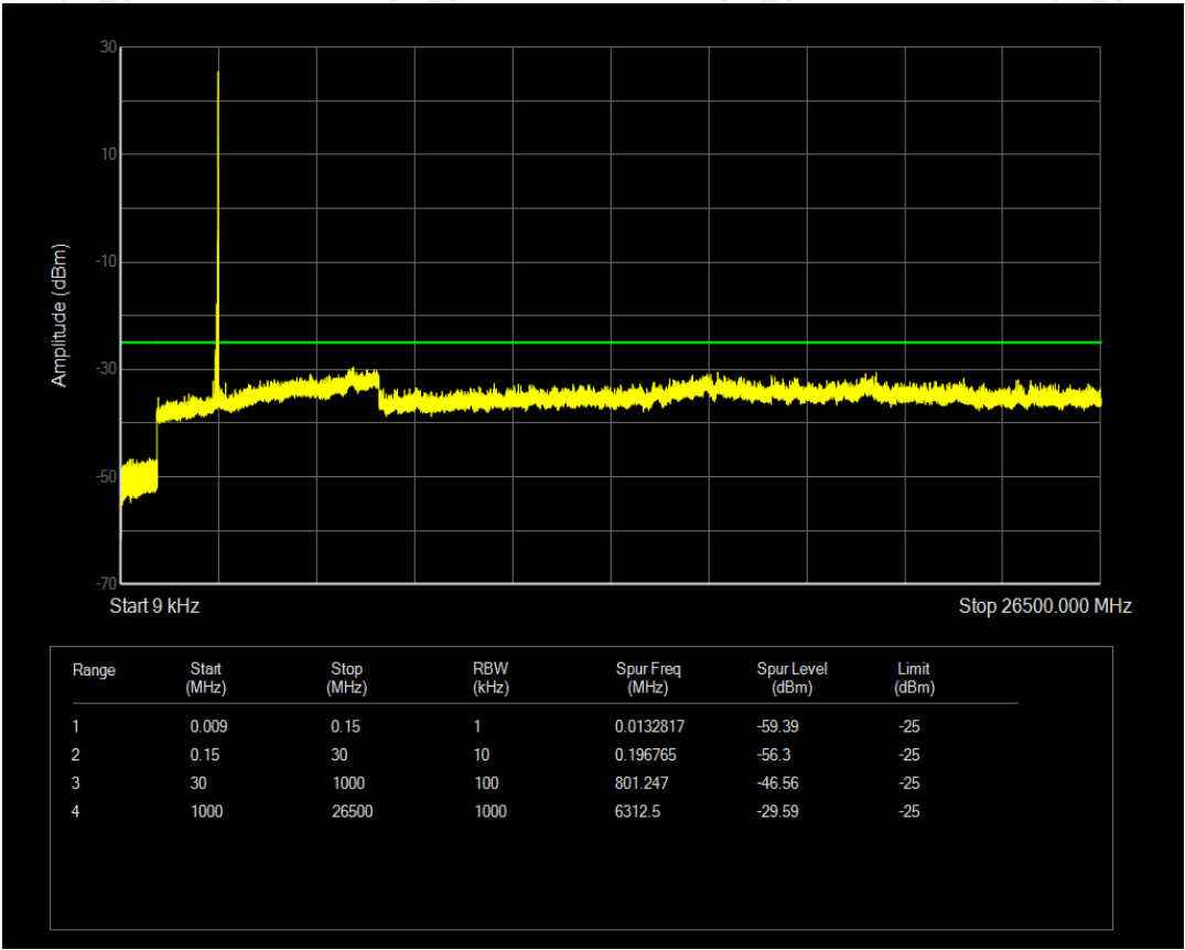
Band41(2545-2655) 16QAM BW=5MHz Channel=41215 RB Size=1 Position=#0
