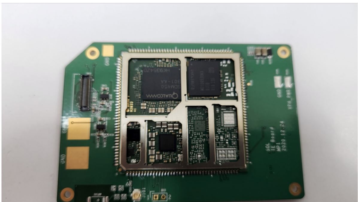
WiFi Board Front(Remove the shield can)
