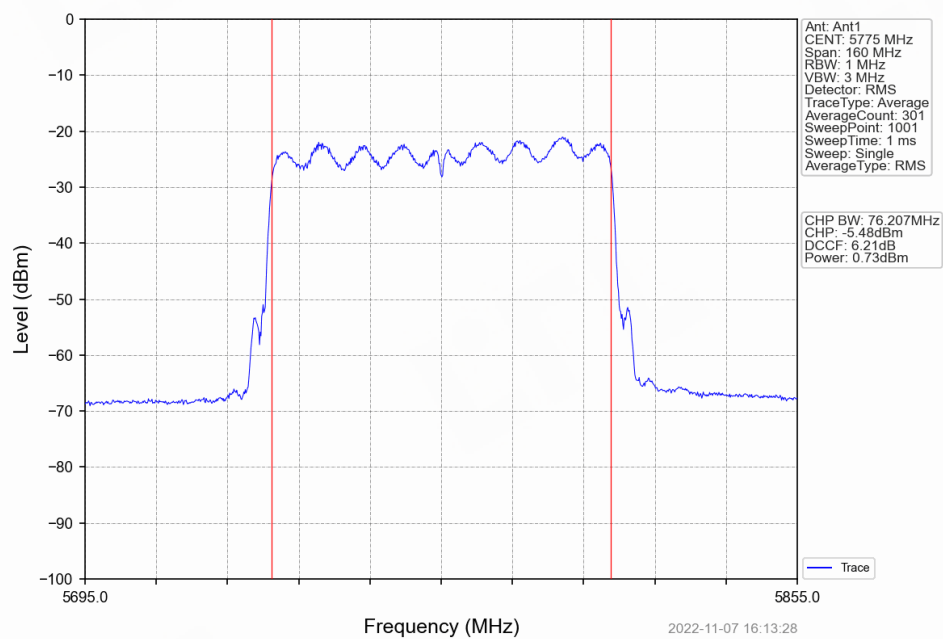
802.11ac(VHT80)_MCH_5775MHz_Ant1_NTV
