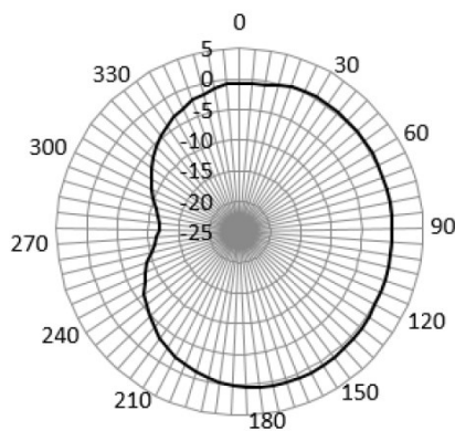
XY-912MHz
