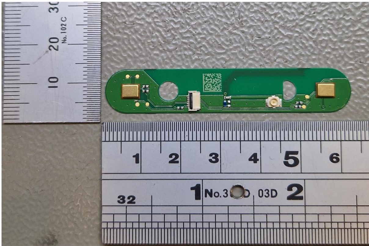
Space Recorder Mic PCBA top side.
