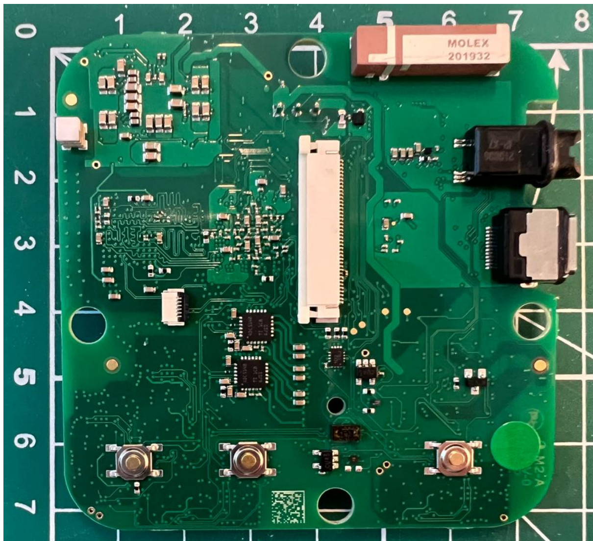
Space Recorder Main PCBA bottom side.
