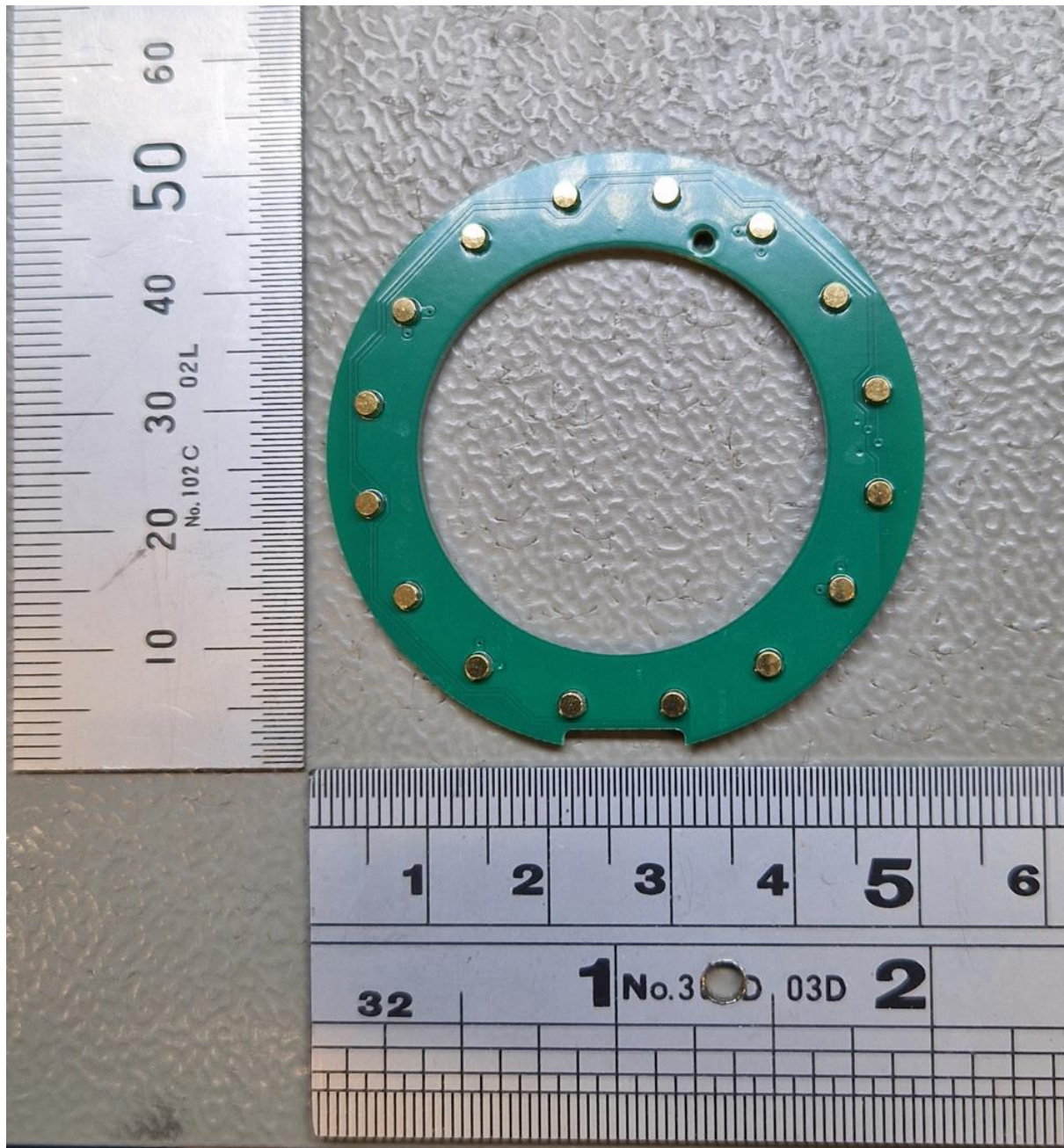
Space Recorder Pogo PCBA top side.
