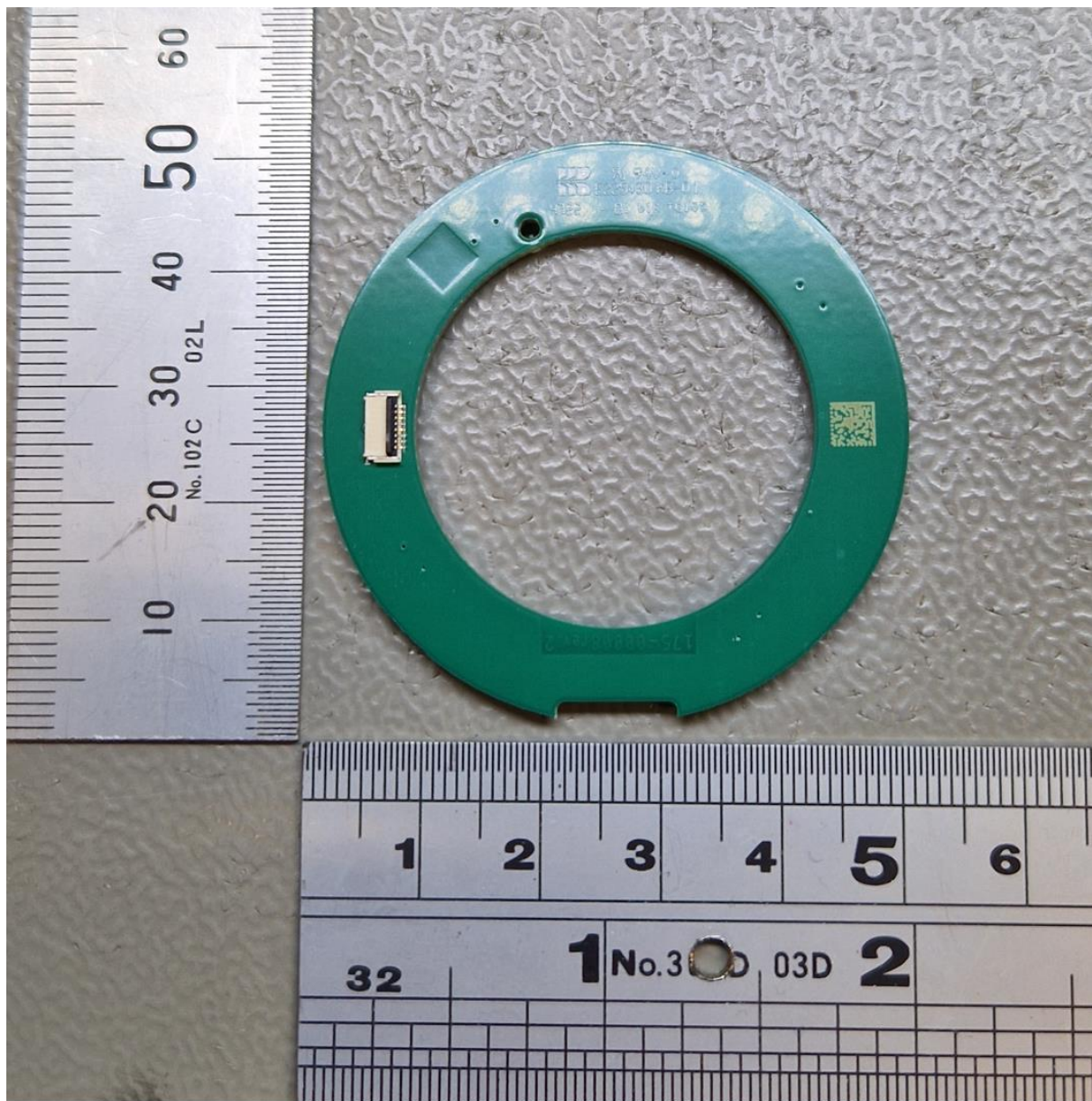
Space Recorder Pogo PCBA bottom side.
