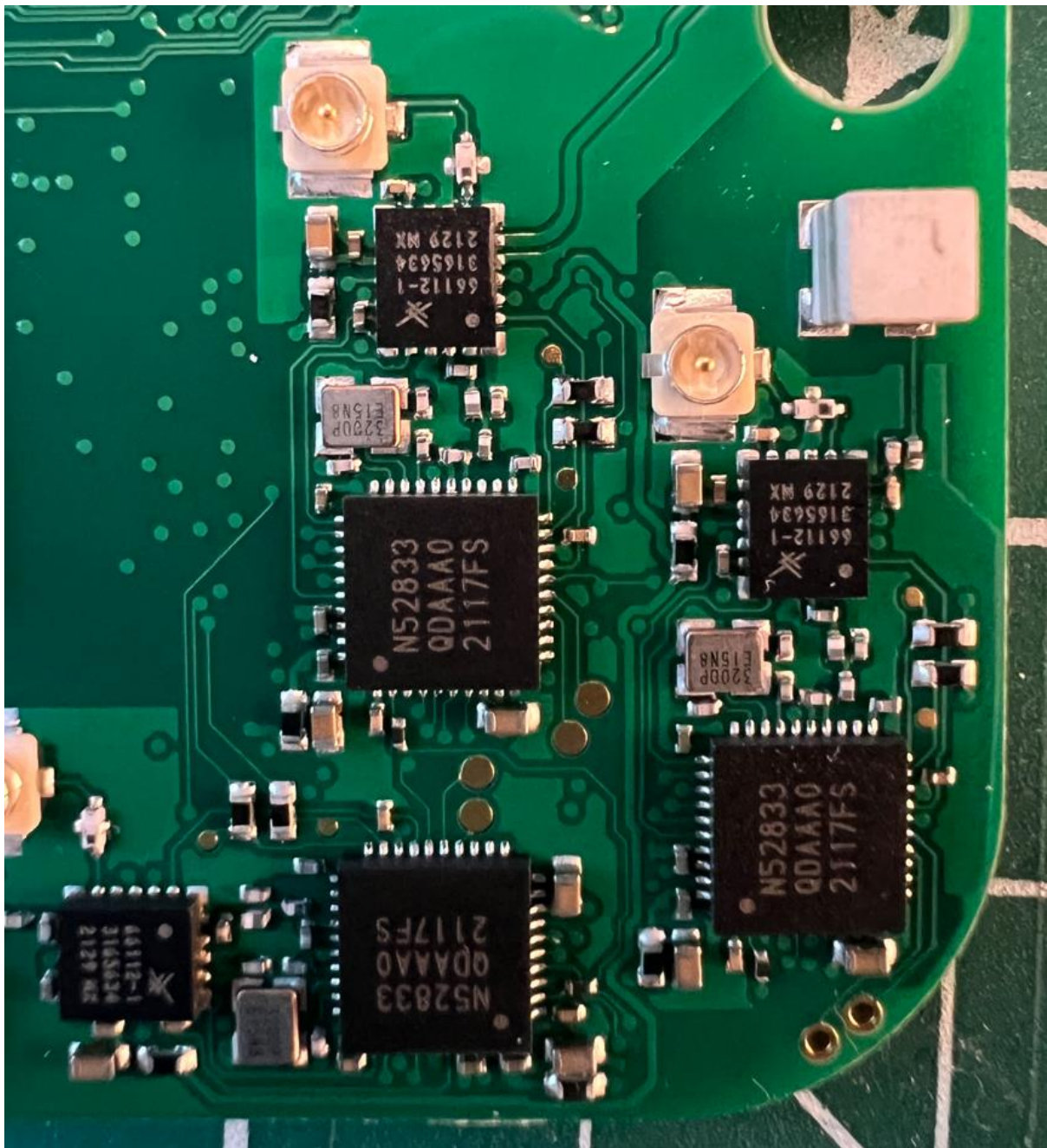
Space Recorder Main top side detail 2
