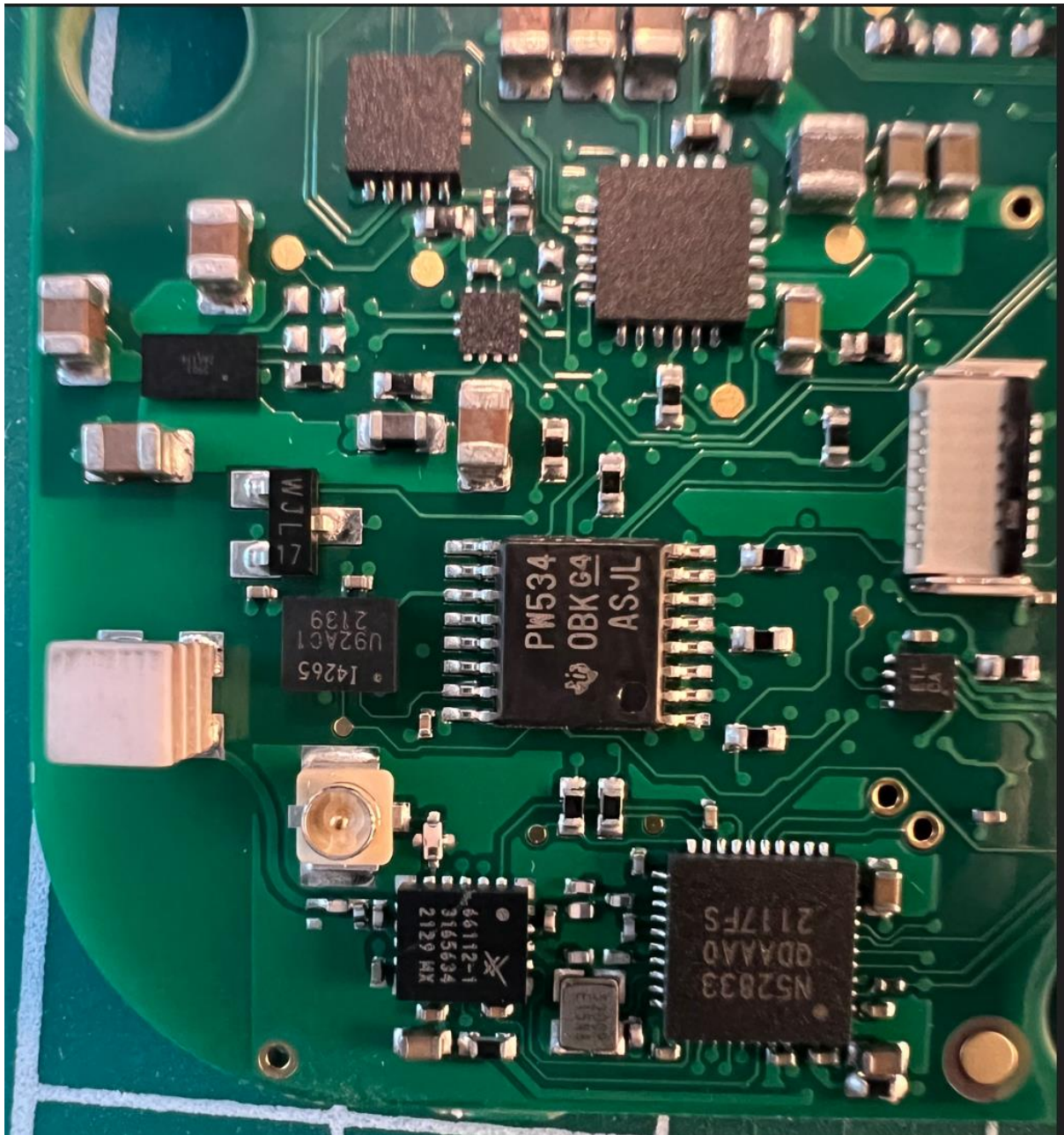
Space Recorder Main top side detail 1
