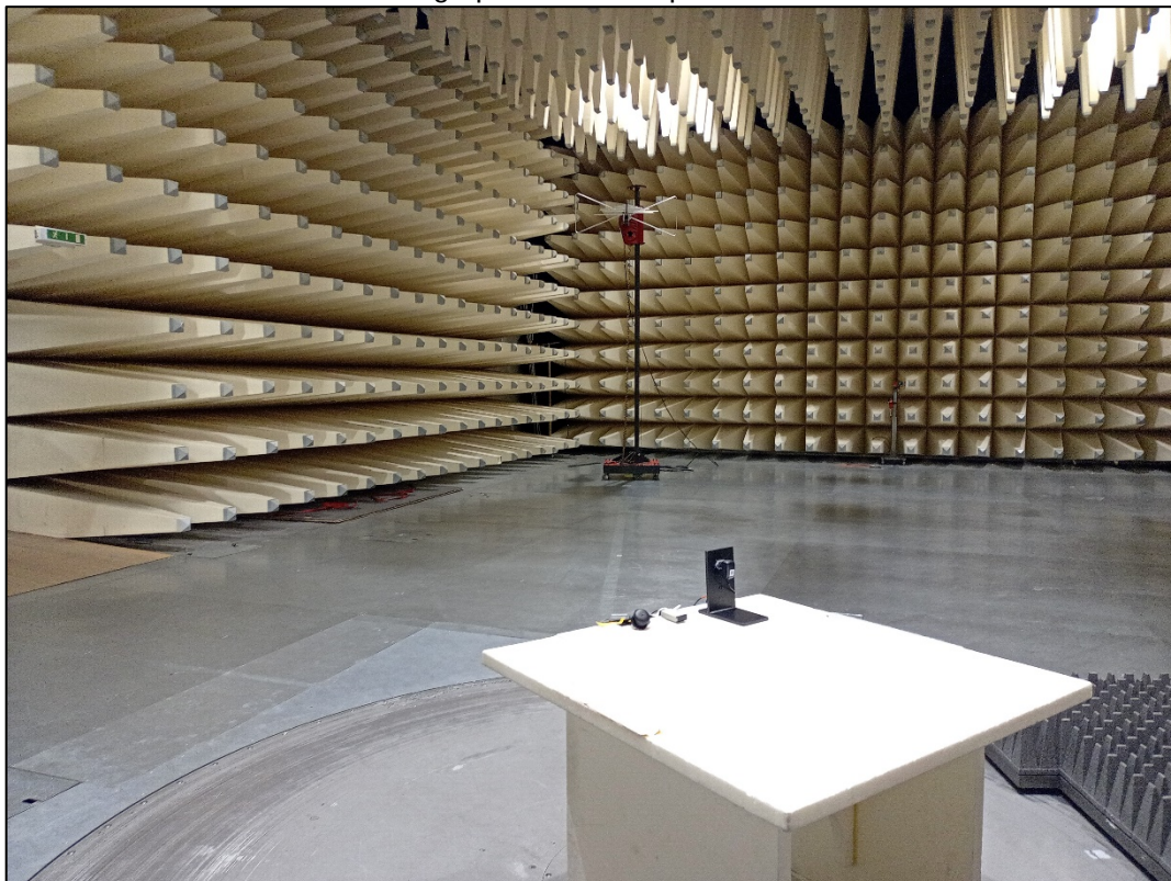
Photo 5: Photograph of Test setup 2 radiated emission
