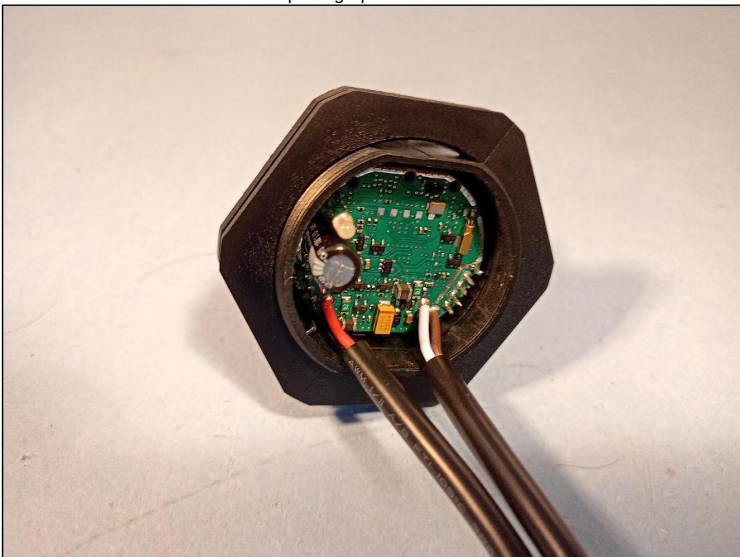
Photo 12: photograph of EUT B rear view
