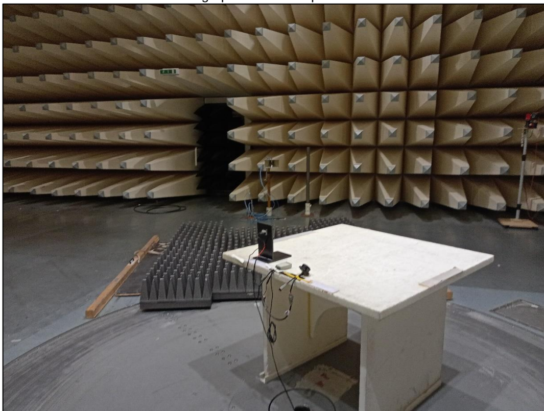
Photo 6: Photograph of Test setup 2 radiated emission
