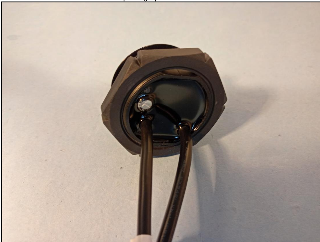
Photo 9: photograph of EUT A rear view
