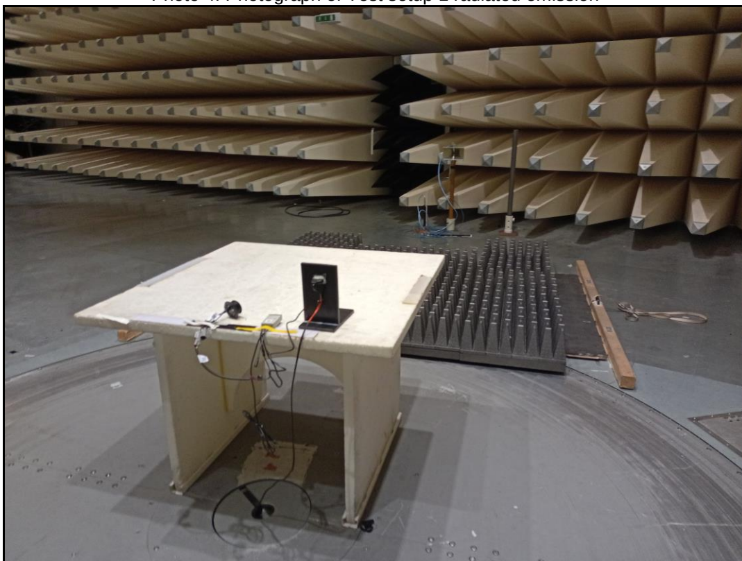
Photo 4: Photograph of Test setup 1 radiated emission
