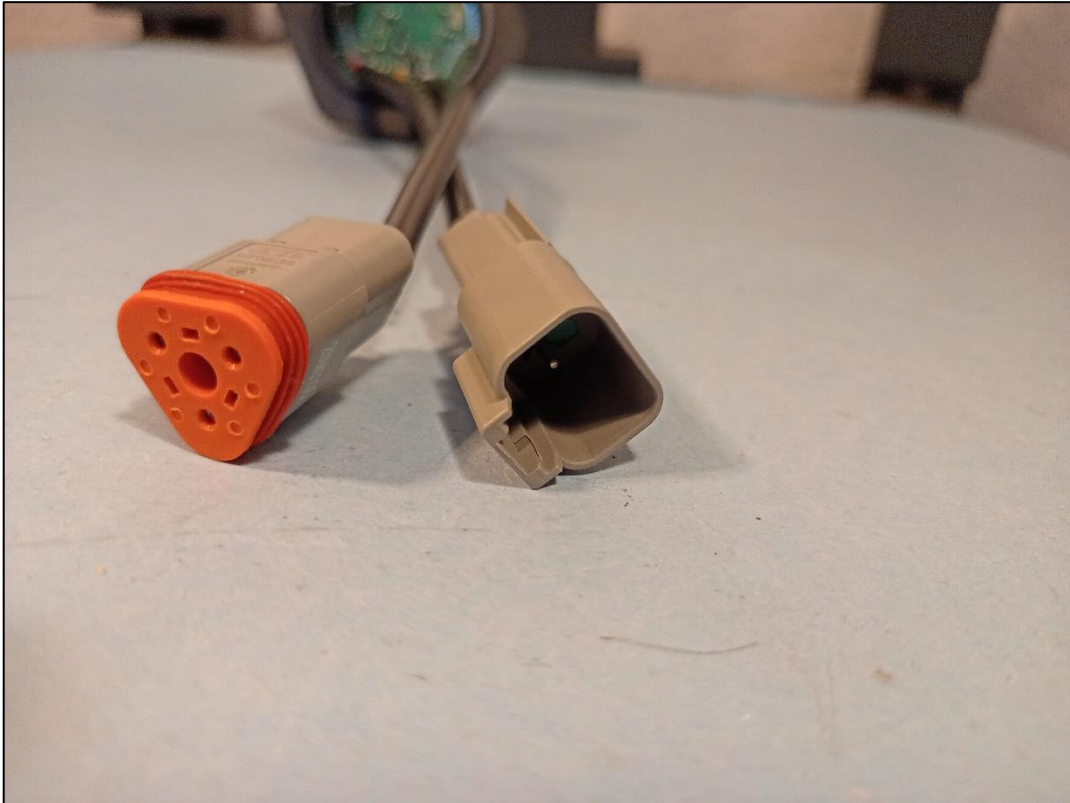
Photo 13: photograph of EUT B connection cables
