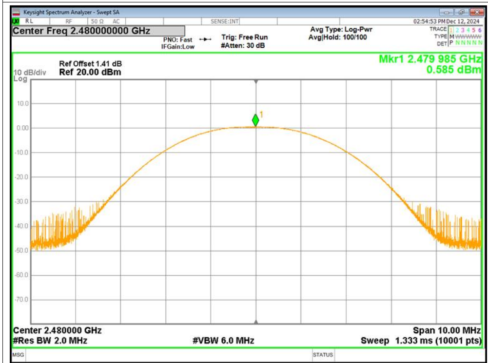
Peak Power NVNT BLE 1M 2480MHz Ant1 Left earphone
