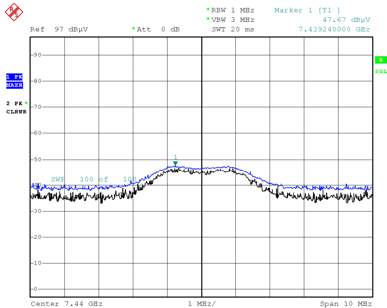
Radiated Spurious Emissions plot – Peak Result (Ch.39 3rd Harmonic, Z-V)
