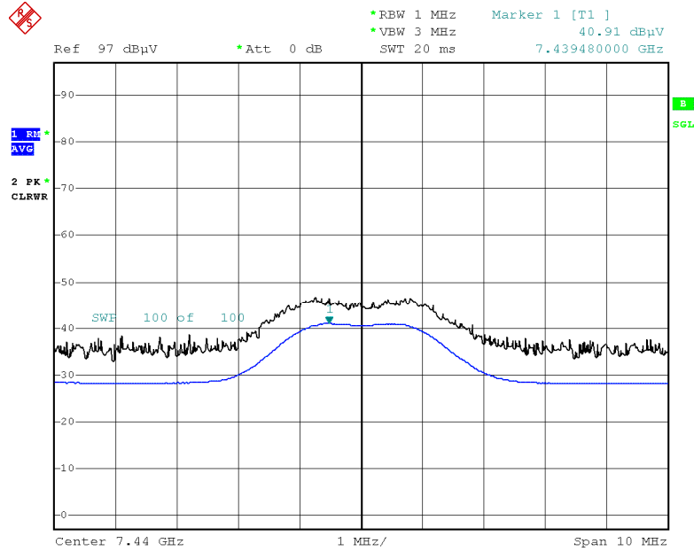
Radiated Spurious Emissions plot – Average Result (Ch.39 3rd Harmonic, Z-V)
