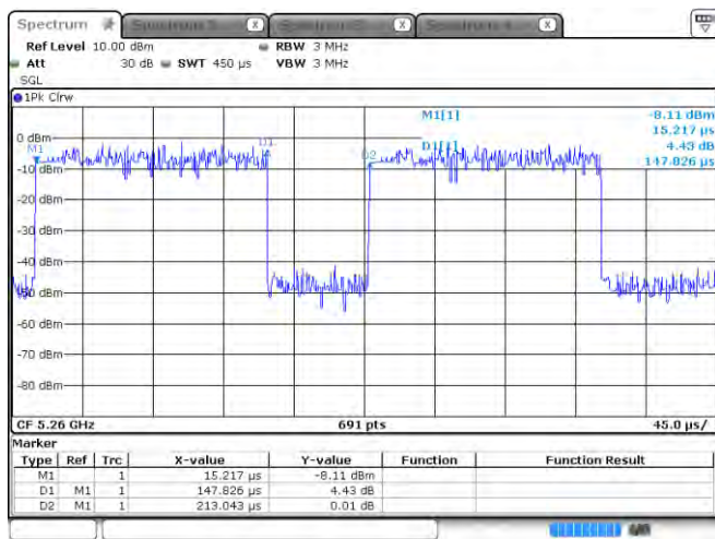
11a 5260 MHz
