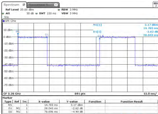
11a 5260 MHz
