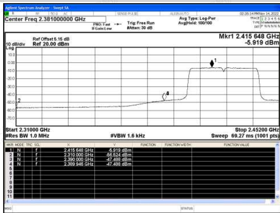
Restrict Band NVNT n40 2422MHz Ant1 Average
