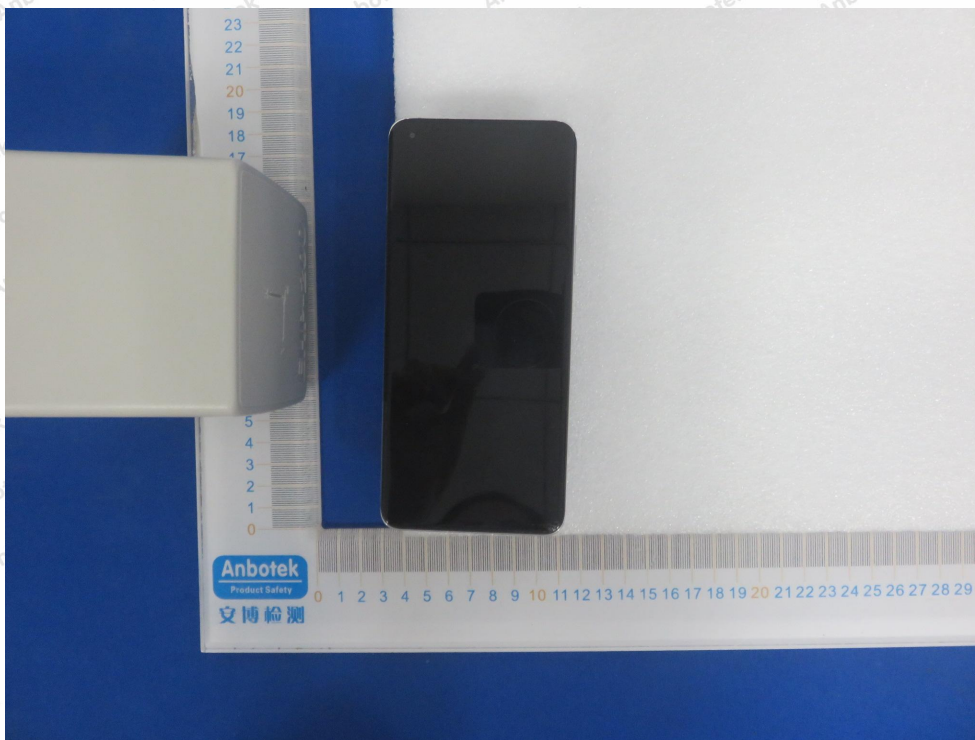
Photo of MPE Measurement at 4 cm
