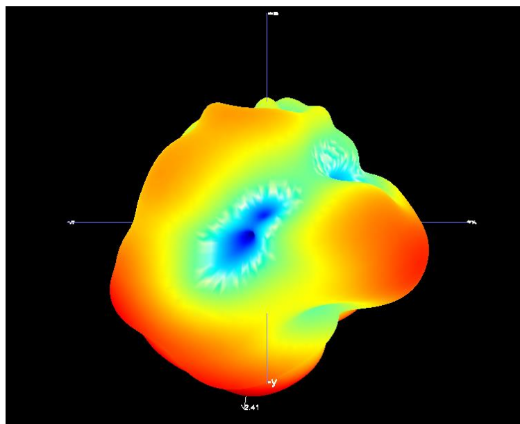
B1.3 3D Pattern for 2500MHz
