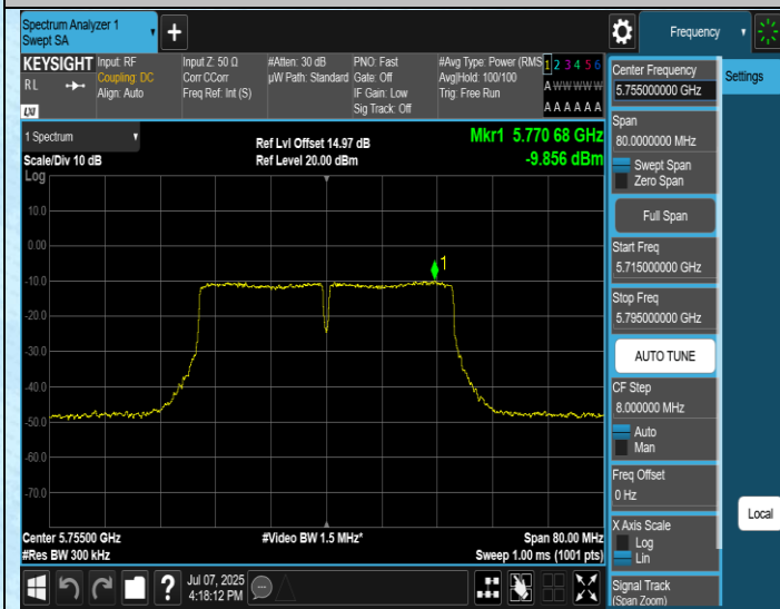
11AC40MIMO-Ant3-5755-PASS
