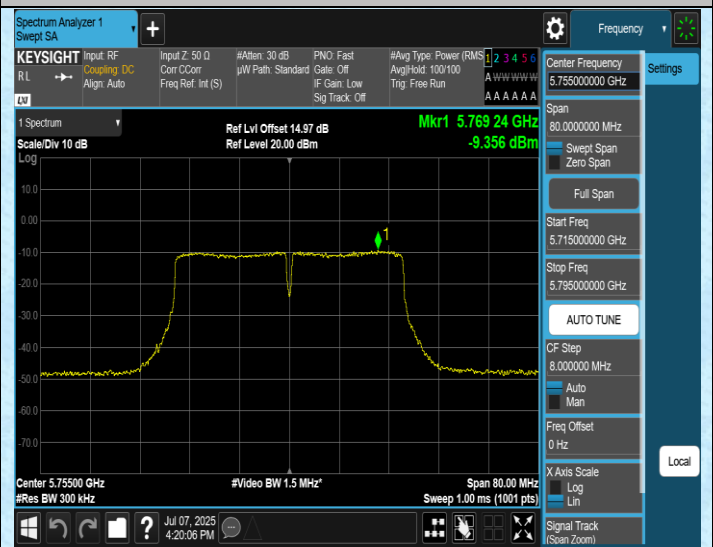
11AC40MIMO-Ant4-5755-PASS
