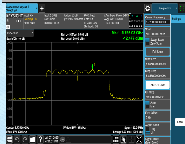
11AC80MIMO-Ant3-5775-PASS
