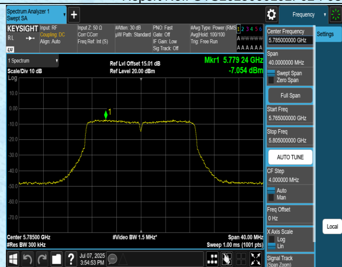
11AC20MIMO-Ant4-5785-PASS
