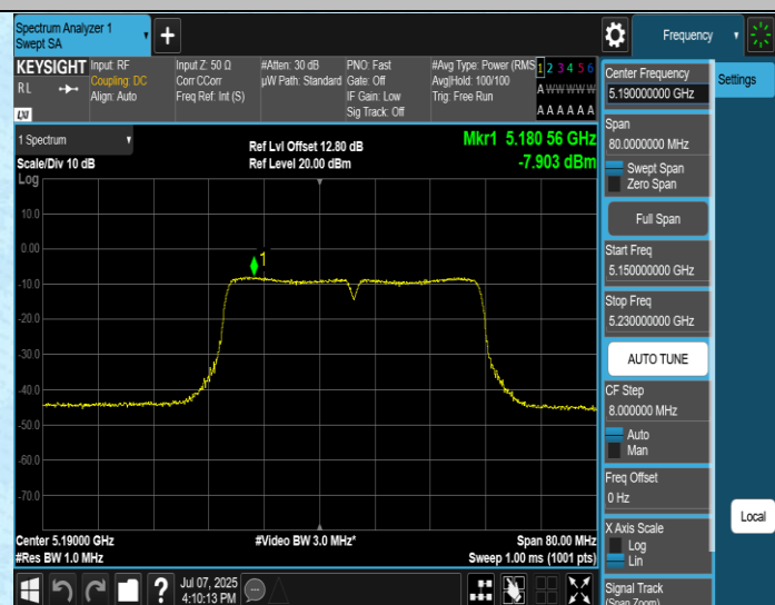
11AC40MIMO-Ant4-5190-PASS
