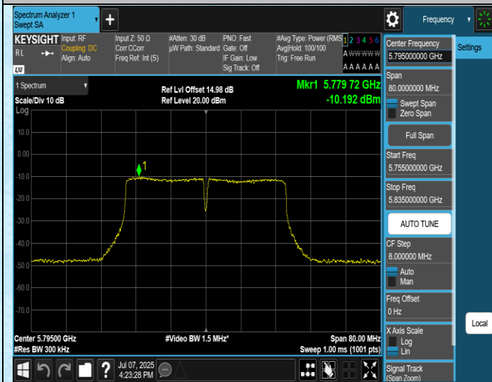
11AC40MIMO-Ant3-5795-PASS
