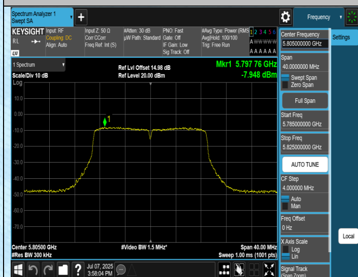
11AC20MIMO-Ant3-5805-PASS
