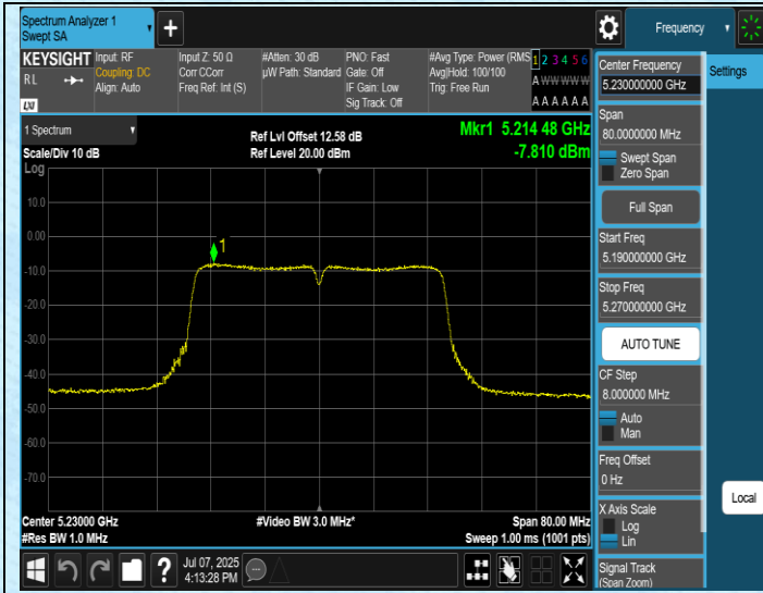
11AC40MIMO-Ant3-5230-PASS
