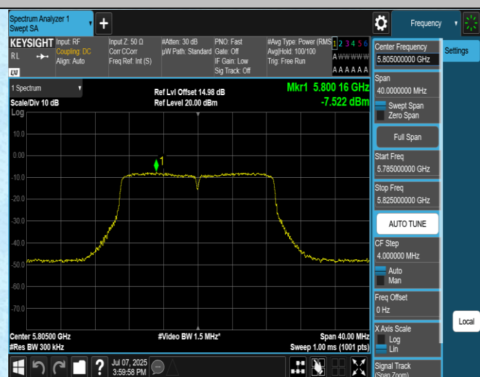
11AC20MIMO-Ant4-5805-PASS
