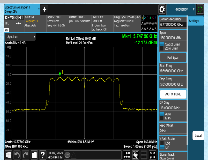
11AC80MIMO-Ant4-5775-PASS
