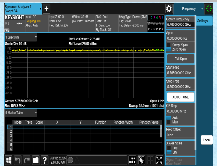
NTNV-11AC20SISO-Ant2-5765
