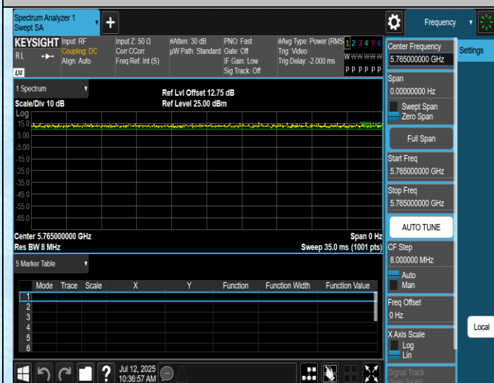
NTNV-11AC20MIMO-Ant1-5765
