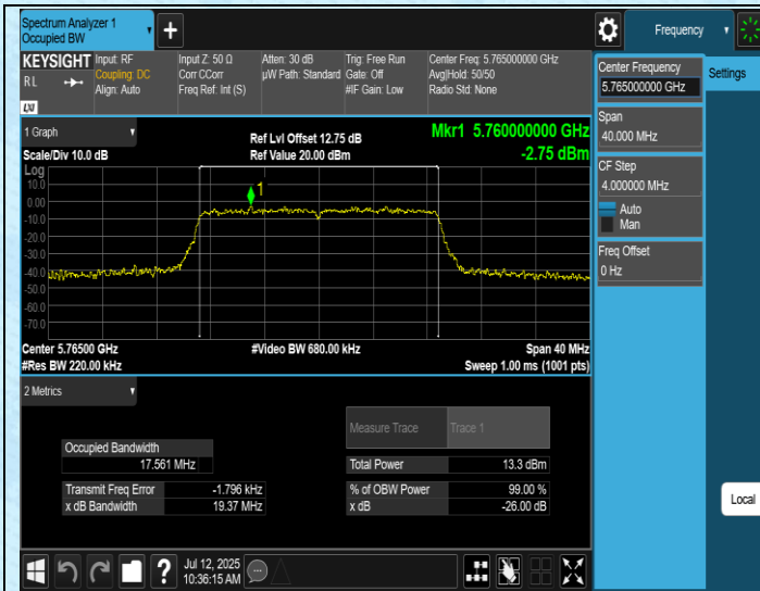
11AC20MIMO-Ant1-5765
