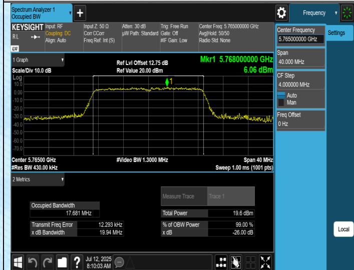
11AC20SISO-Ant1-5765
