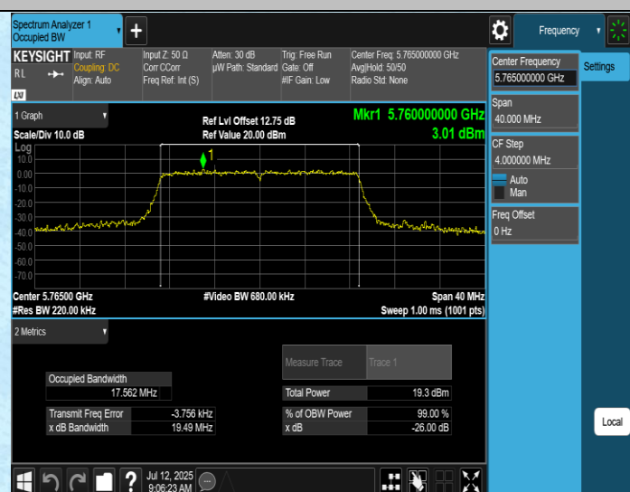
11AC20SISO-Ant2-5765
