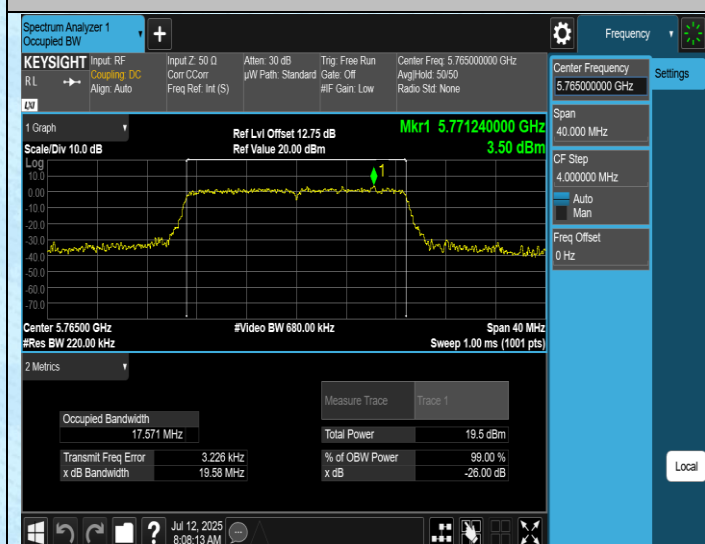
11AC20SISO-Ant1-5765
