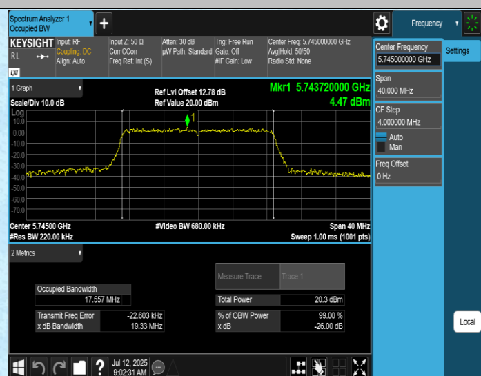
11AC20SISO-Ant2-5745
