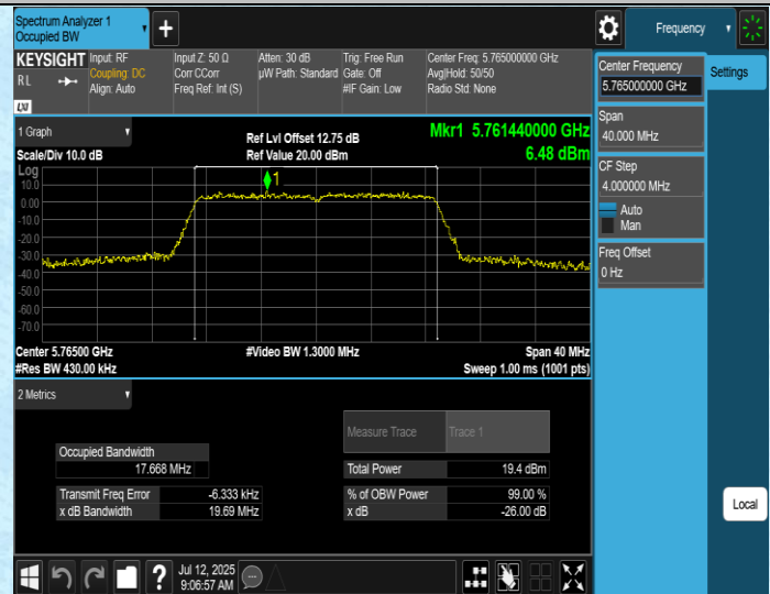
11AC20SISO-Ant2-5765
