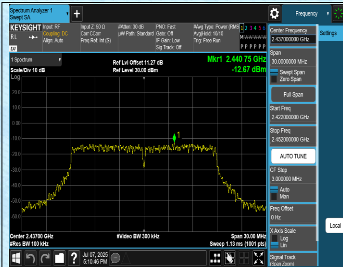
11N20MIMO-Ant3-2437-0~Reference-PASS
