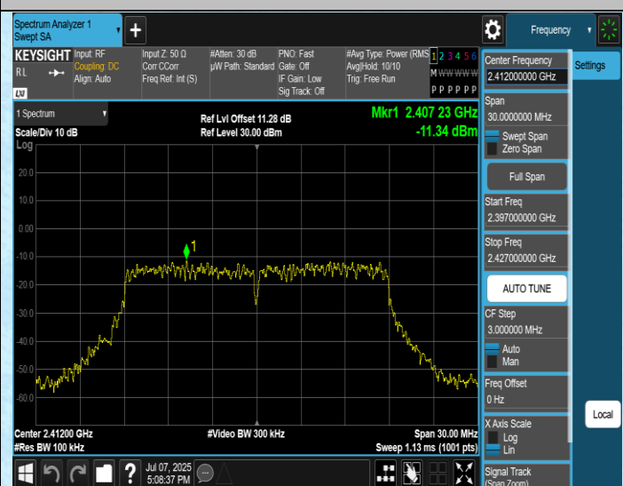
11N20MIMO-Ant4-2412-0~Reference-PASS
