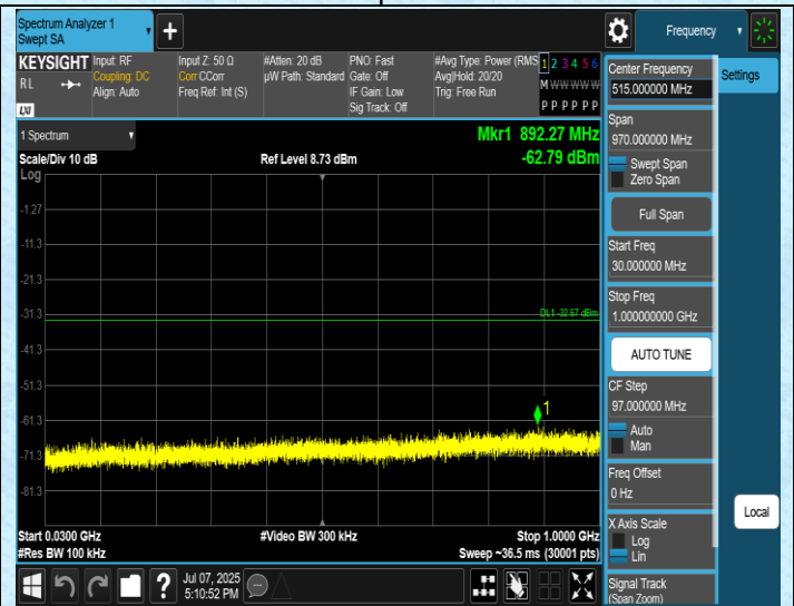
11N20MIMO-Ant3-2437-30~1000-PASS
