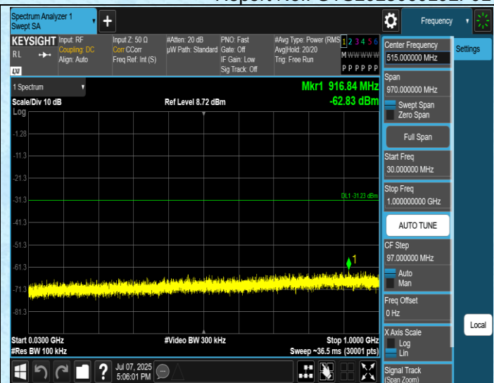
11N20MIMO-Ant3-2412-30~1000-PASS
