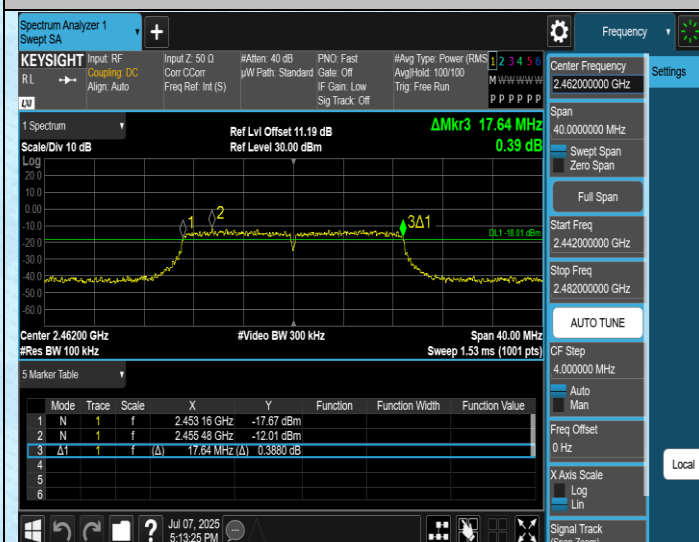
11N20MIMO-Ant3-2462-PASS
