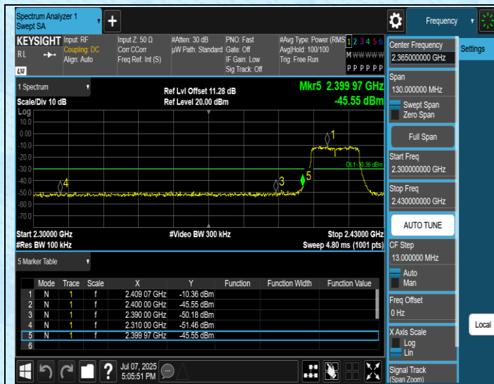
11N20MIMO-Ant3-2412-PASS
