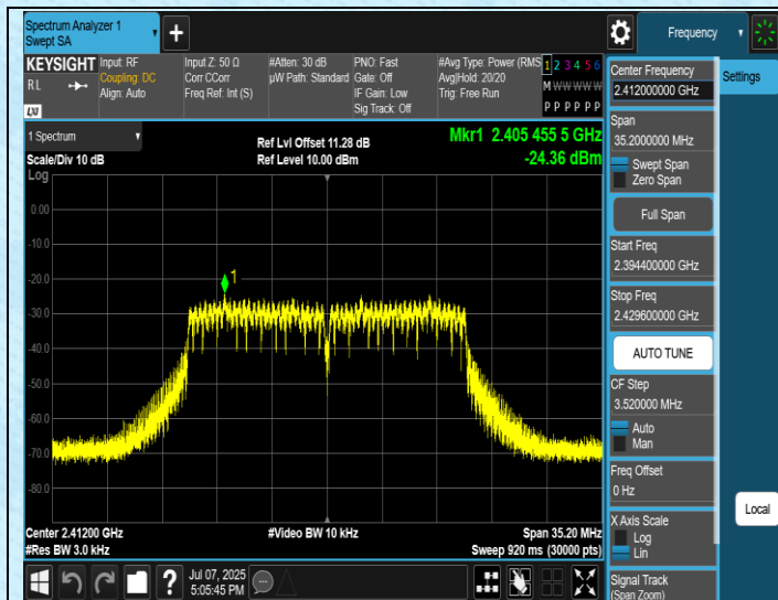
11N20MIMO-Ant3-2412-PASS
