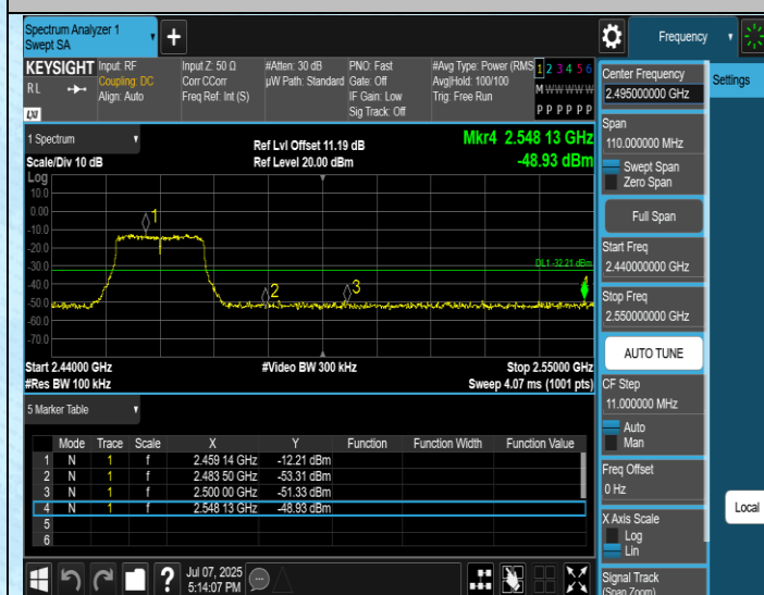
11N20MIMO-Ant3-2462-PASS
