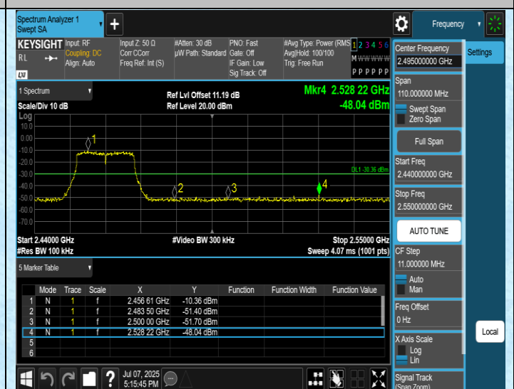
11N20MIMO-Ant4-2462-PASS
