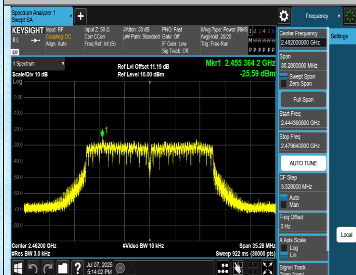
11N20MIMO-Ant3-2462-PASS
