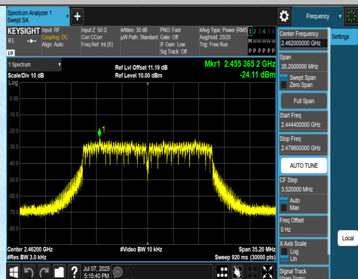
11N20MIMO-Ant4-2462-PASS
