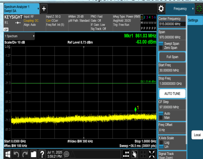
11N20MIMO-Ant1-2437-30~1000-PASS
