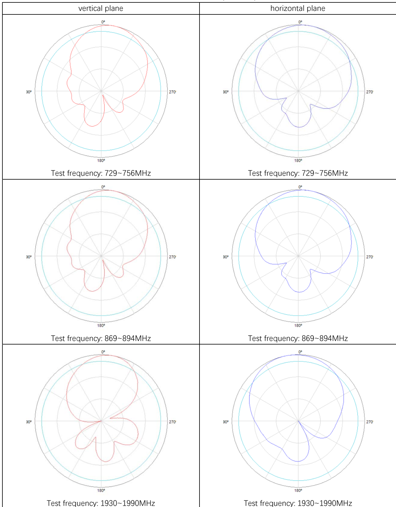
Panle antenna ambient temperature pattern
