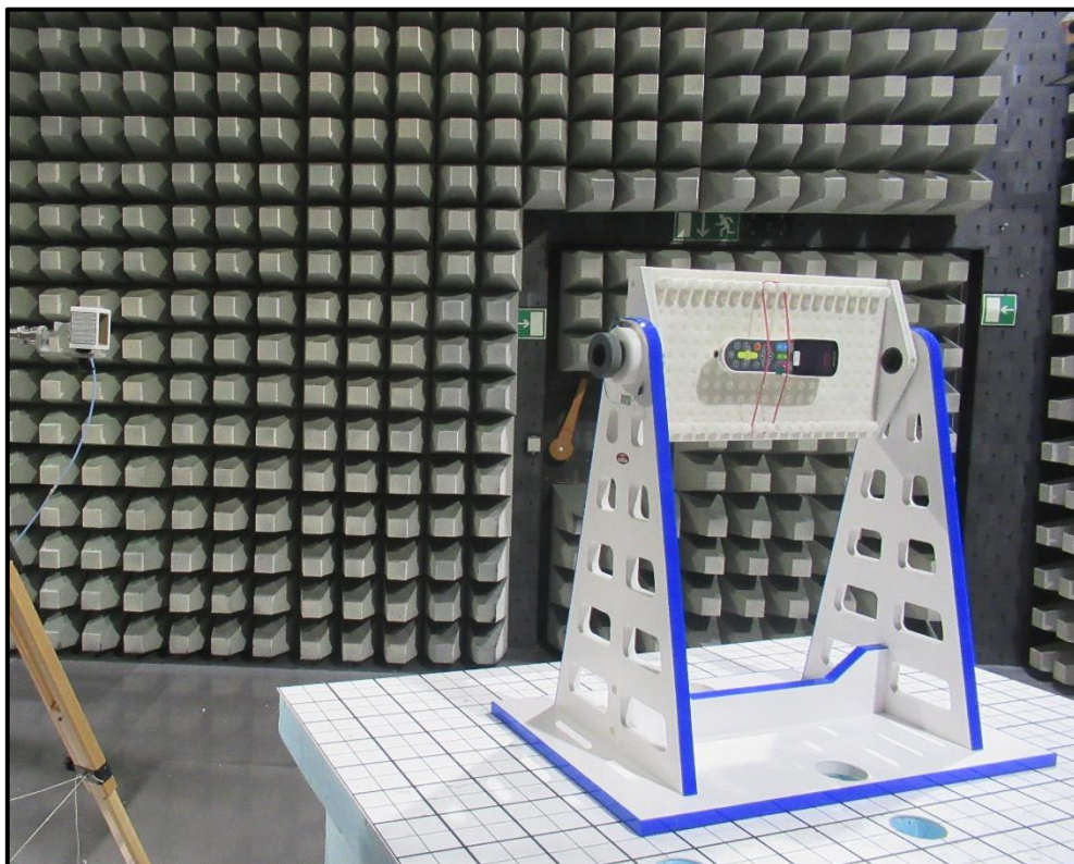
Photo 8 Radiated Test Setup above 18 GHz
