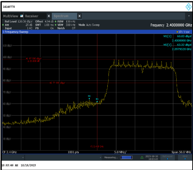
Lower Band Edge Peak Measurement
