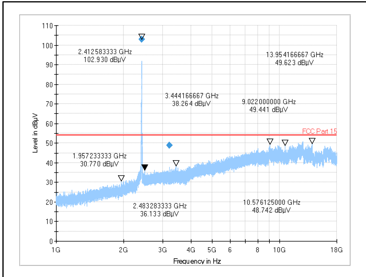
Plot: 1 GHz – 18GHz: 802.11b / 20 MHz / 1 Mbps / PWR MAX / Bottom Channel
