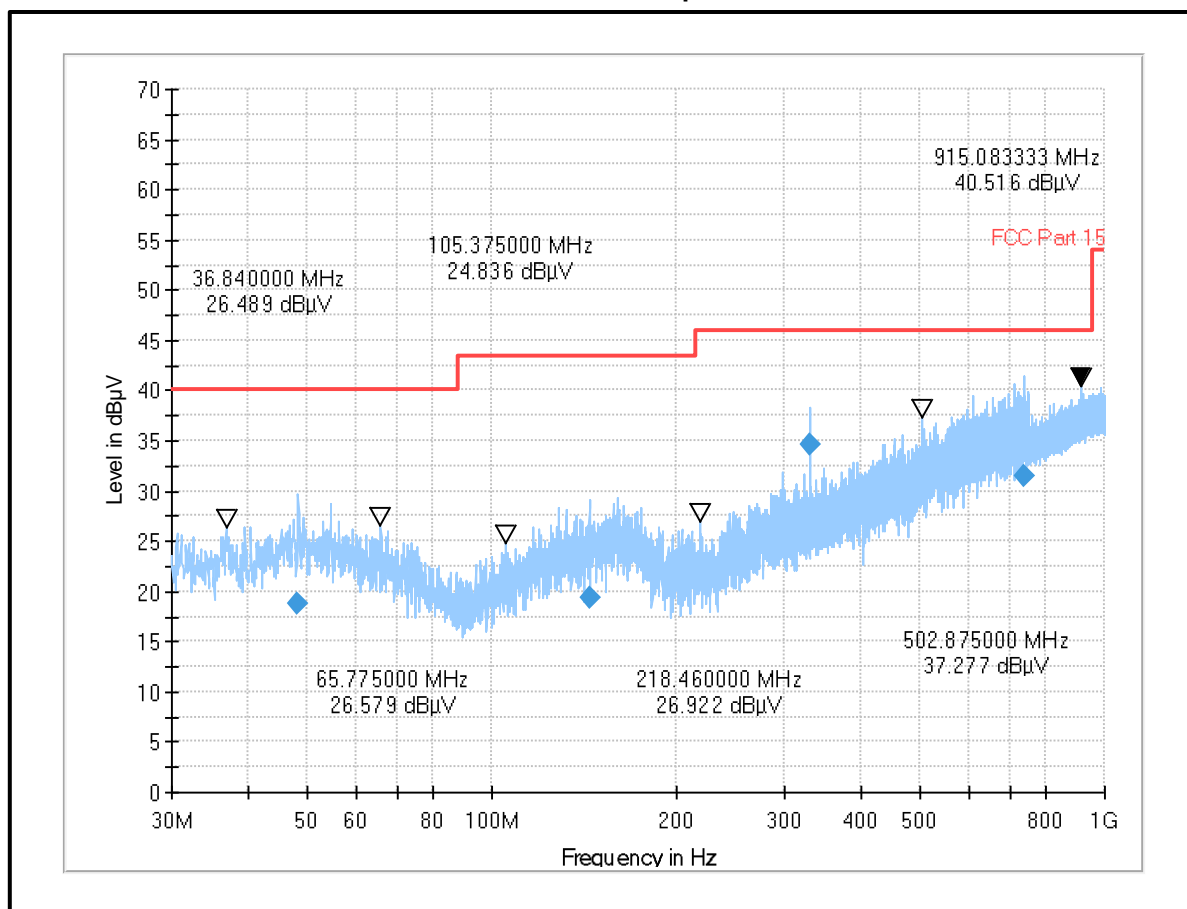
Plot: 30 MHz – 1GHz: 802.11b / 20 MHz / 1 Mbps / PWR MAX / Bottom Channel
