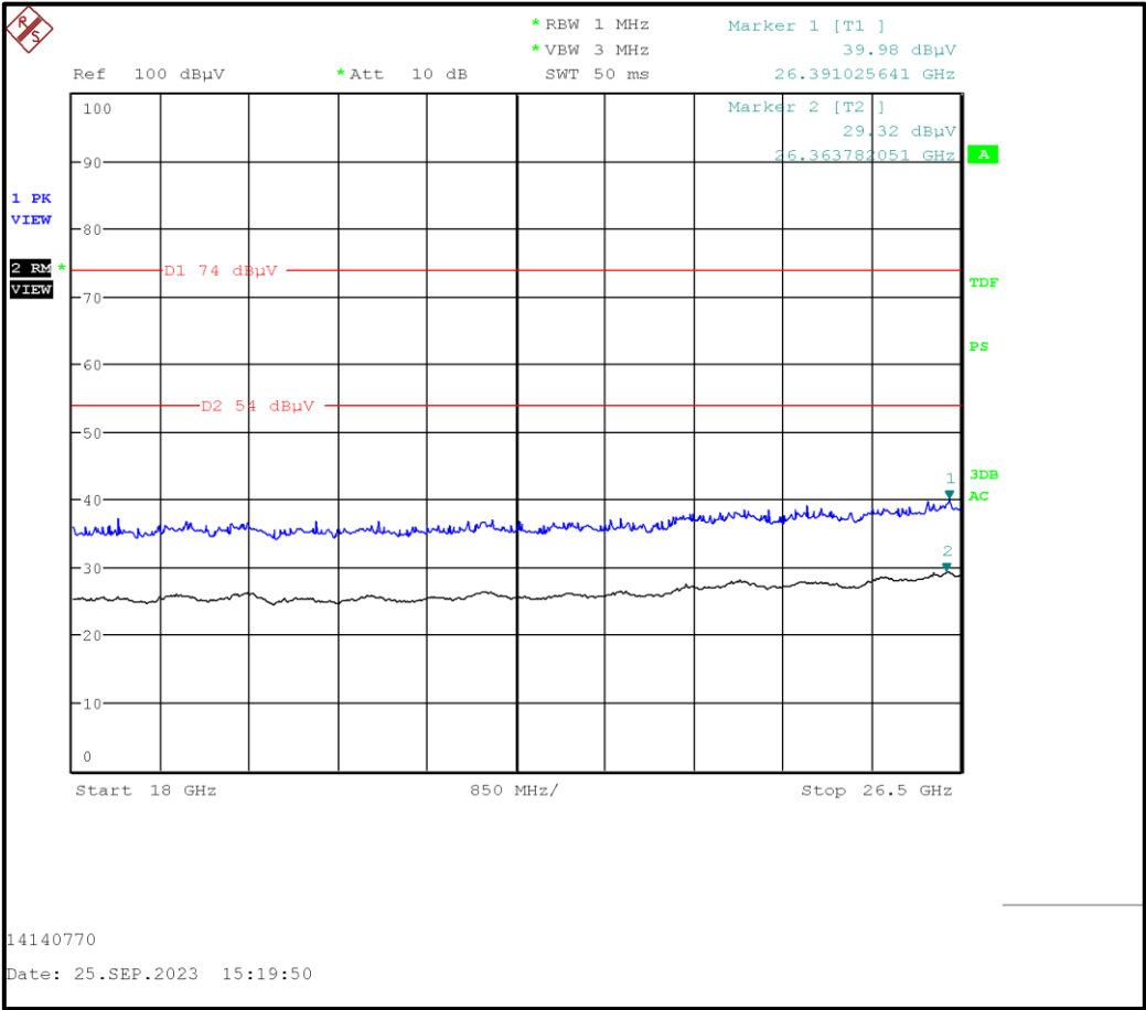
Plot: 18 GHz – 26.5 GHz: 802.11b / 20 MHz / 1 Mbps / PWR MAX / Bottom Channel
