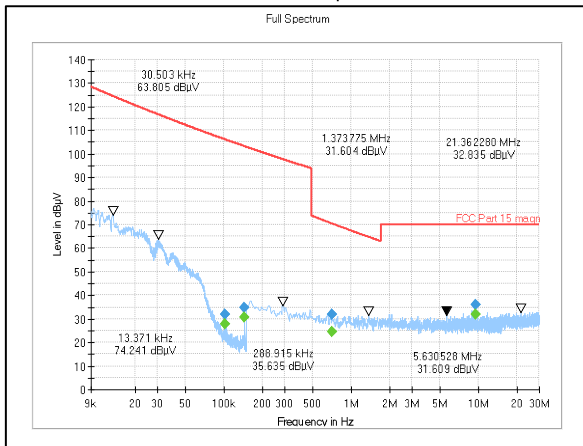
Plot: 9 kHz – 30 MHz: 802.11b / 20 MHz / 1 Mbps / PWR MAX / Bottom Channel
