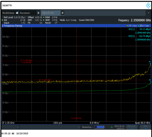
2310 MHz to 2390 MHz Restricted Band Plot
