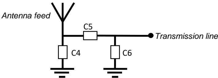
Matching circuit
