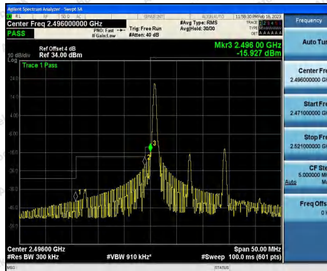
Band41-15MHz-16QAM-39725-1RB#74
