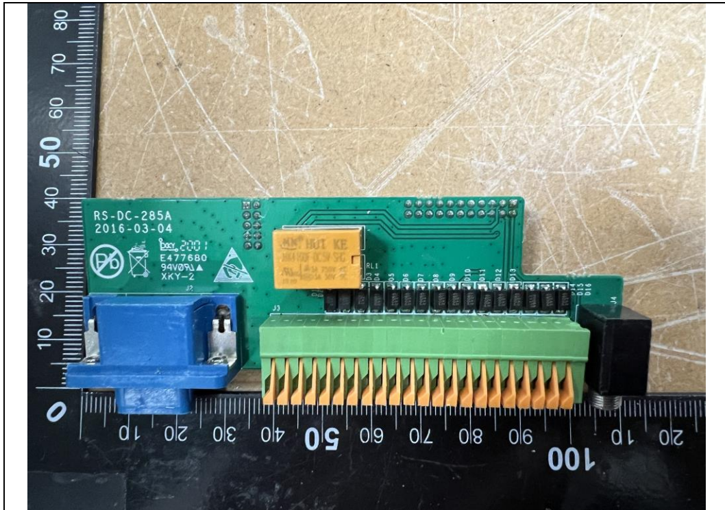
NX22-516KRS4_Sub Board2 Front
