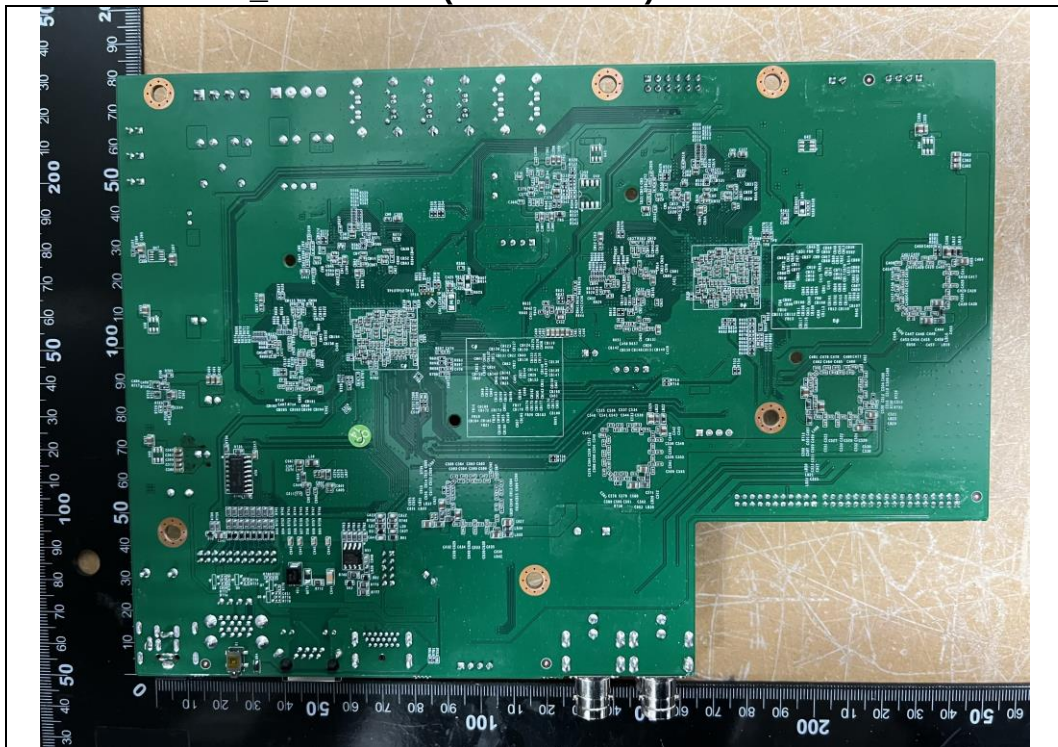
NX22-516KRS4_Main Board(RS-DM-466B) Front Rear
