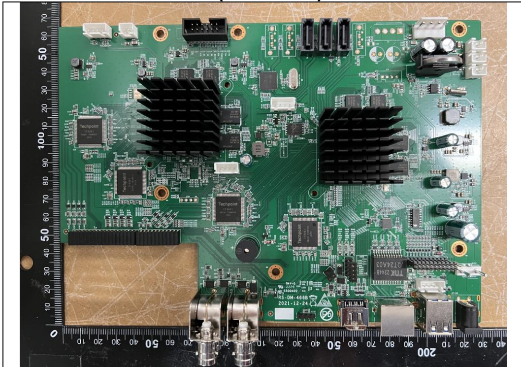
NX22-516KRS4_Main Board(RS-DM-466B) Front
