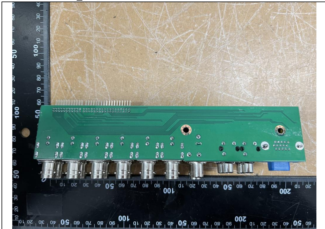
NX22-516KRS4_Sub Board1 Rear
