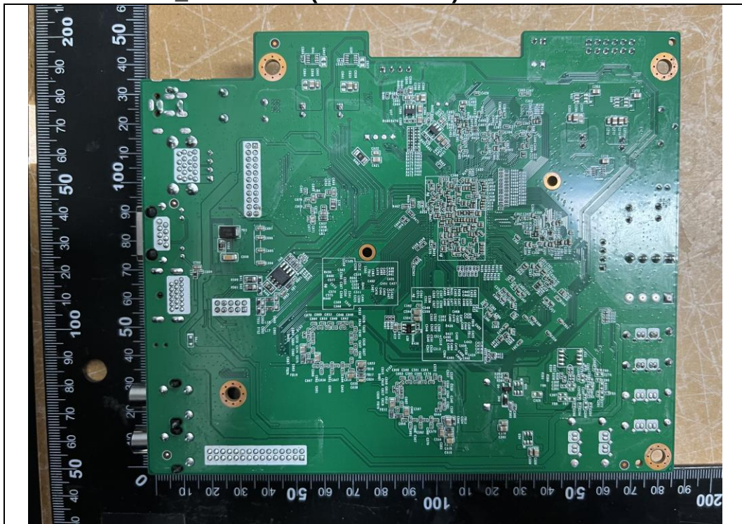
NX20-508KRS4_Main Board(RS-DM-445A) Front Rear
