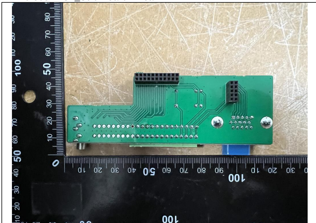
NX20-508KRS4_Sub Board1 Rear
