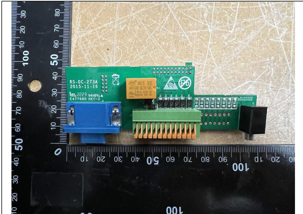
NX20-508KRS4_Sub Board1 Front
