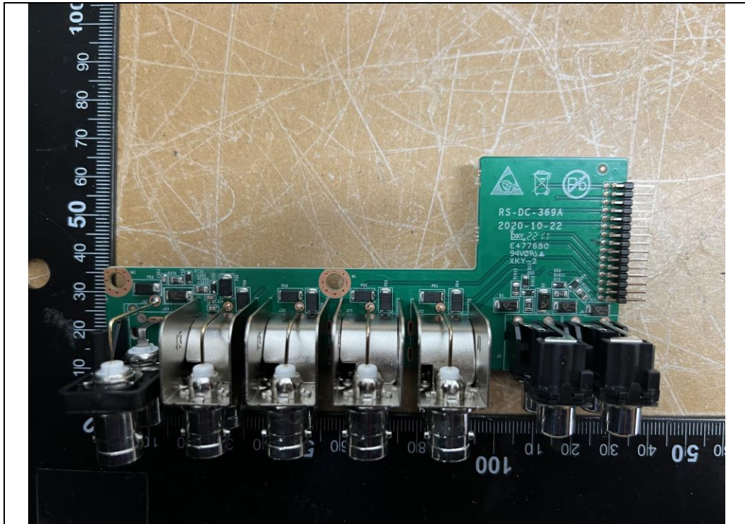
NX20-508KRS4_Sub Board2 Front
