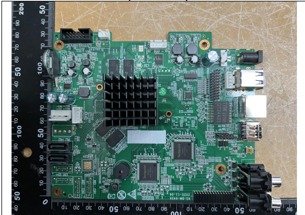
NX20-508KRS4_Main Board(RS-DM-445A) Front
