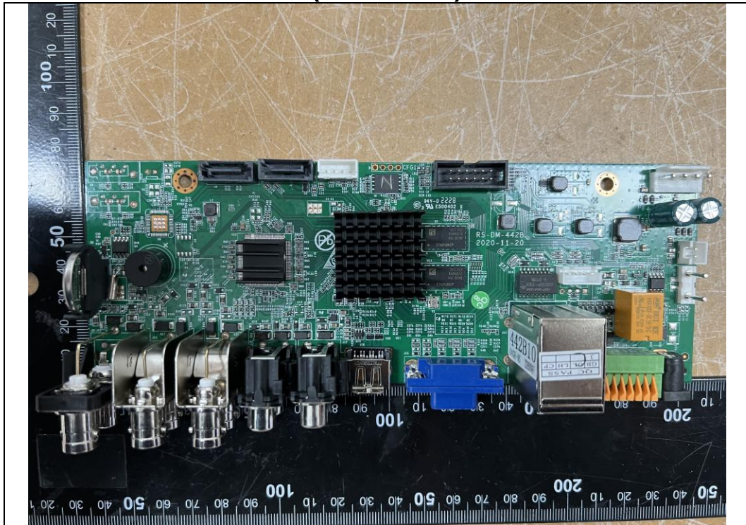
HX20-504KRS4_Main Board(RS-DM-442B) Front
