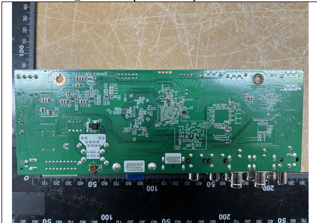
HX20-504KRS4_Main Board(RS-DM-442B) Front Rear
