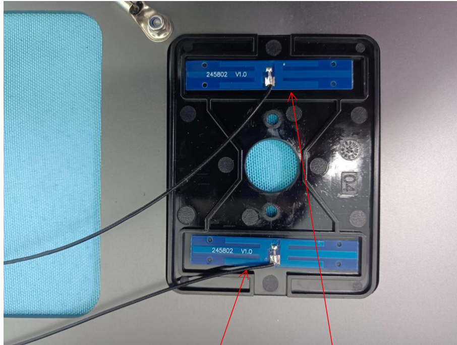
WiFi-ANT1 WiFi-ANT2
