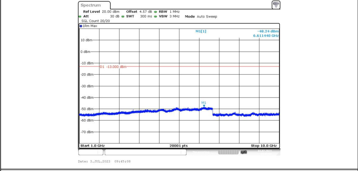
Band5-4183-4-1000~10000MHz
