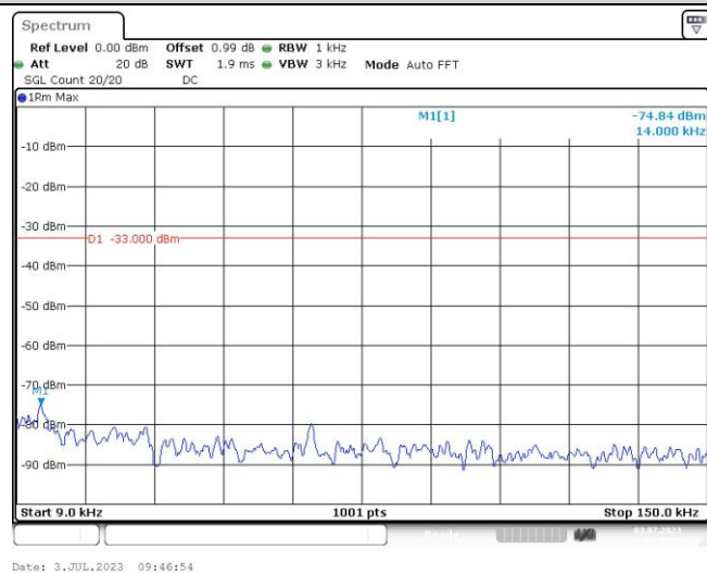
Band5-4183-1-0.009~0.15MHz
