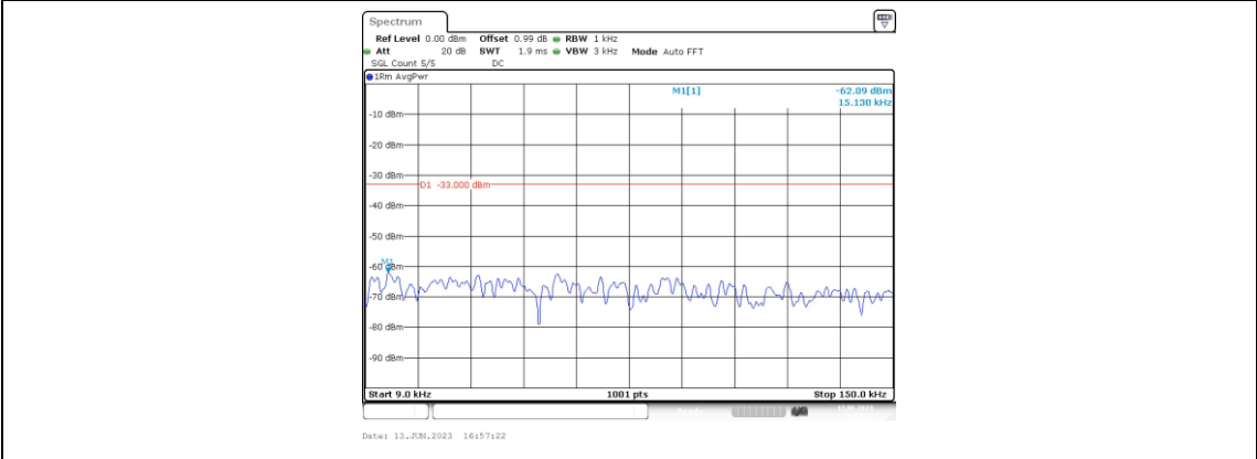
Band66-20MHz-QPSK-132572-1RB#0-Range1:0.009~0.15MHz
