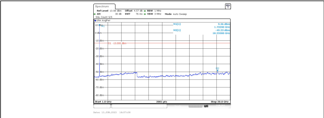
Band66-20MHz-16QAM-132322-1RB#0-Range4:1000~20000MHz
