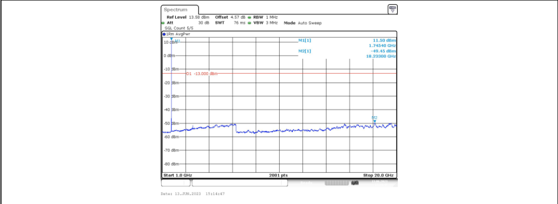
Band66-5MHz-QPSK-132322-1RB#0-Range4:1000~20000MHz
