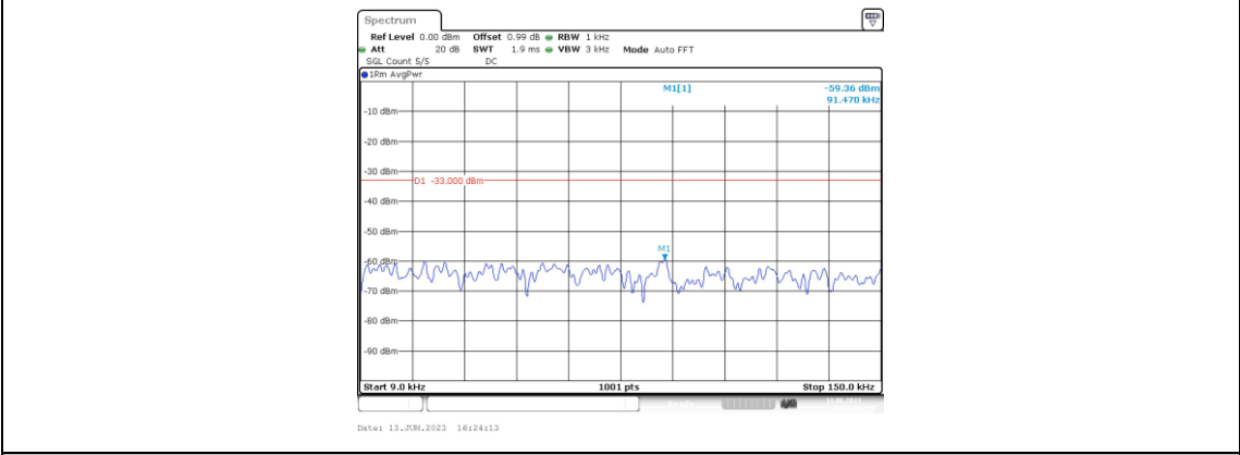
Band66-15MHz-16QAM-132597-1RB#0-Range1:0.009~0.15MHz
