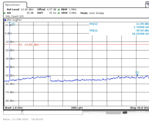
Band66-15MHz-QPSK-132322-1RB#0-Range4:1000~20000MHz
