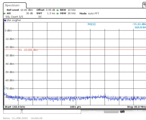
Band66-3MHz-16QAM-132657-1RB#0-Range2:0.15~30MHz
