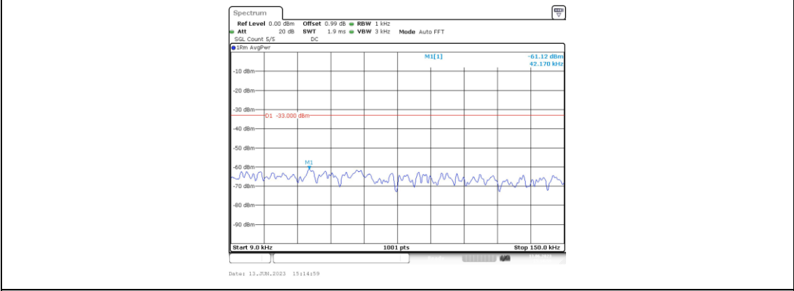
Band66-5MHz-16QAM-132322-1RB#0-Range1:0.009~0.15MHz
