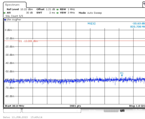
Band66-10MHz-16QAM-132322-1RB#0-Range3:30~1000MHz
