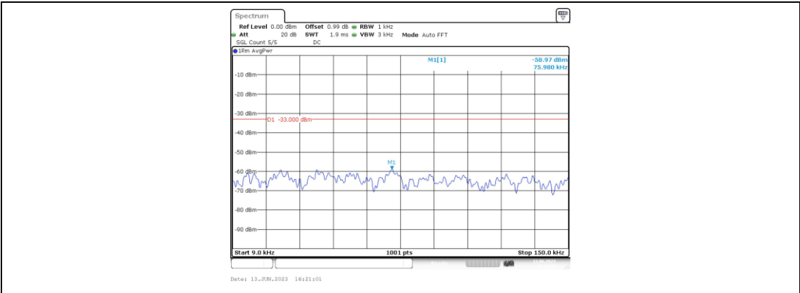
Band66-15MHz-16QAM-132047-1RB#0-Range1:0.009~0.15MHz
