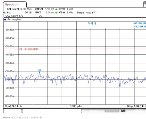
Band66-10MHz-QPSK-132622-1RB#0-Range1:0.009~0.15MHz
