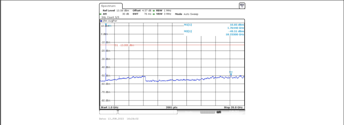
Band66-15MHz-QPSK-132597-1RB#0-Range4:1000~20000MHz
