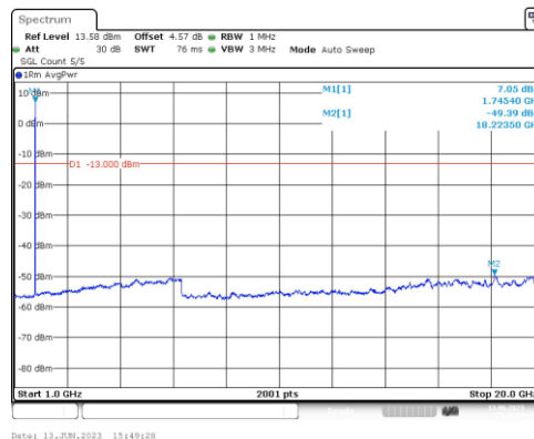
Band66-10MHz-16QAM-132322-1RB#0-Range4:1000~20000MHz
