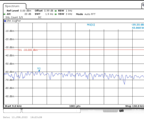
Band66-15MHz-QPSK-132597-1RB#0-Range1:0.009~0.15MHz
