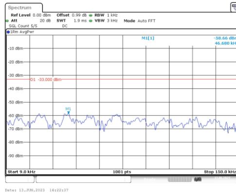
Band66-15MHz-16QAM-132322-1RB#0-Range1:0.009~0.15MHz
