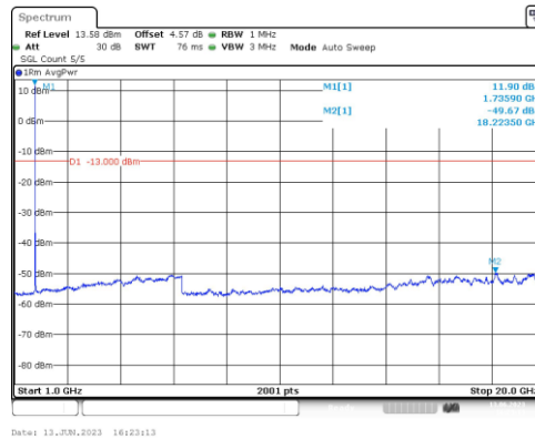
Band66-15MHz-16QAM-132322-1RB#0-Range4:1000~20000MHz
