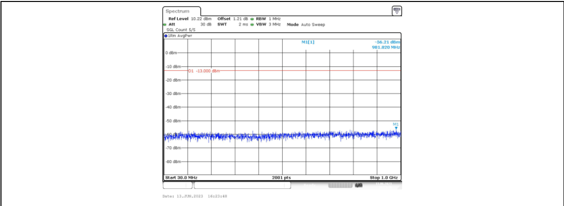
Band66-15MHz-QPSK-132597-1RB#0-Range3:30~1000MHz
