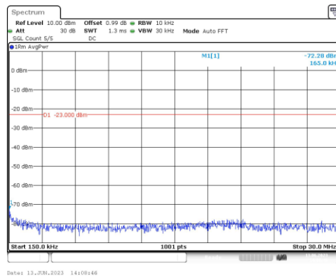
Band66-1.4MHz-QPSK-132665-1RB#0-Range2:0.15~30MHz
