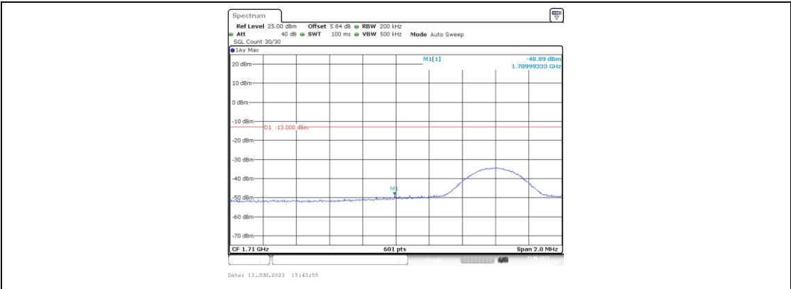
Band66-10MHz-QPSK-132022-1RB#49
