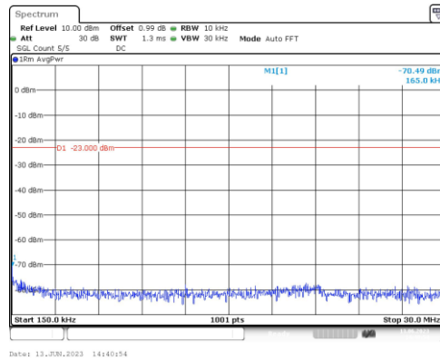
Band66-3MHz-16QAM-132322-1RB#0-Range2:0.15~30MHz
