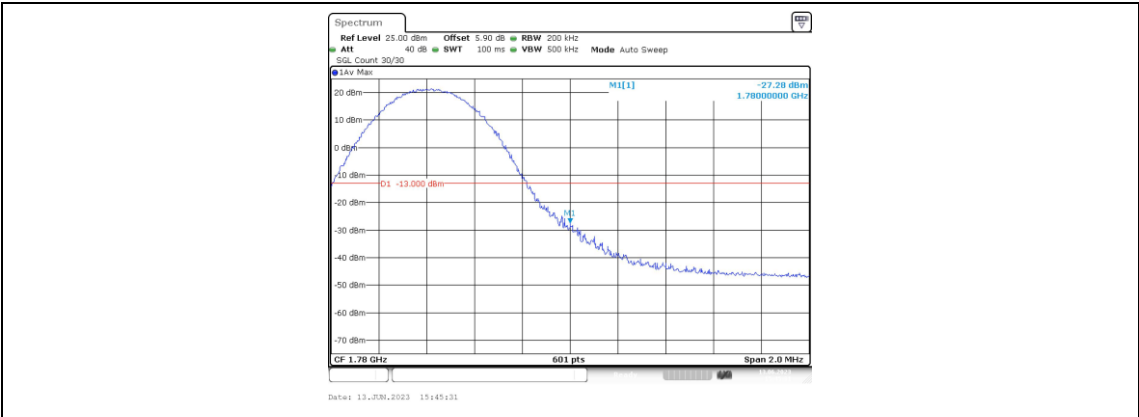
Band66-10MHz-16QAM-132622-1RB#49
