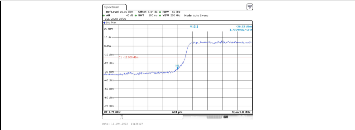
Band66-3MHz-16QAM-131987-15RB#0
