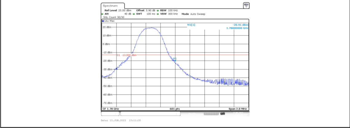
Band66-5MHz-16QAM-132647-1RB#24
