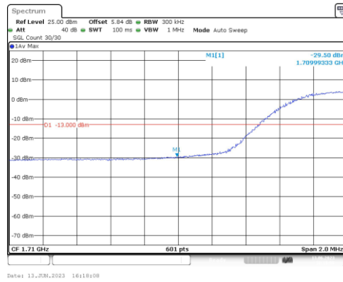
Band66-15MHz-QPSK-132047-75RB#0
