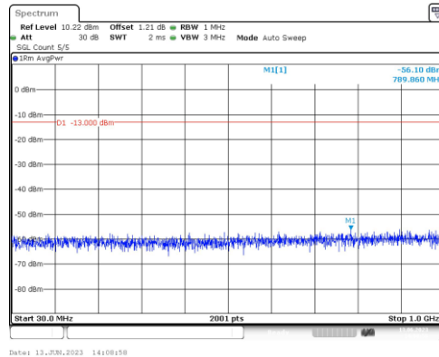
Band66-1.4MHz-QPSK-132665-1RB#0-Range3:30~1000MHz
