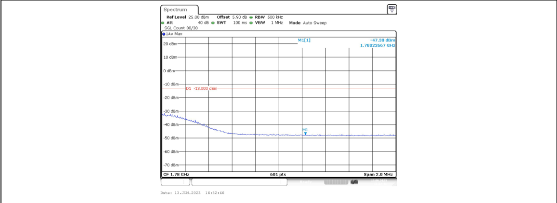
Band66-20MHz-16QAM-132572-1RB#0
