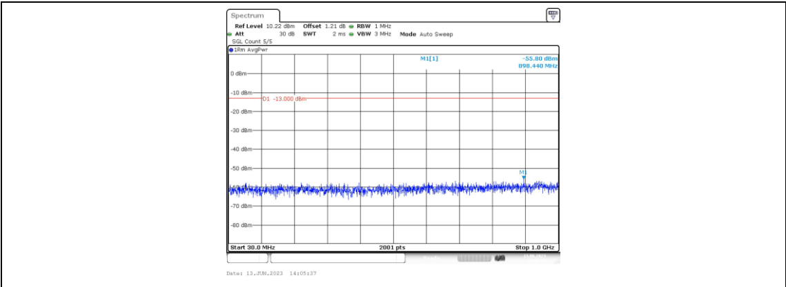
Band66-1.4MHz-QPSK-131979-1RB#0-Range3:30~1000MHz
