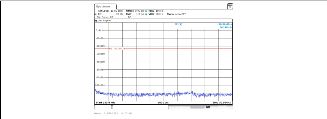
Band66-1.4MHz-QPSK-132322-1RB#0-Range2:0.15~30MHz
