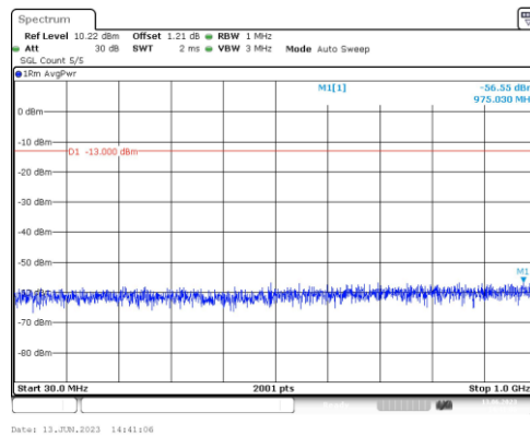
Band66-3MHz-16QAM-132322-1RB#0-Range3:30~1000MHz
