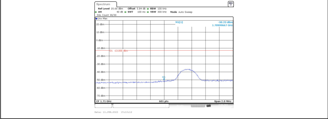
Band66-5MHz-QPSK-131997-1RB#24
