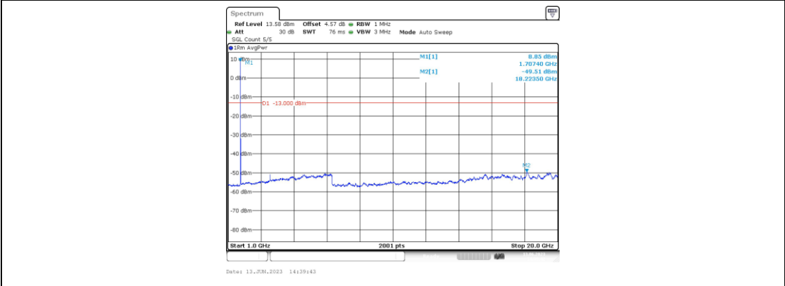
Band66-3MHz-16QAM-131987-1RB#0-Range4:1000~20000MHz
