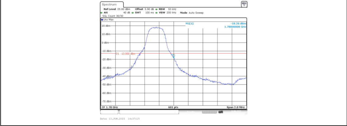
Band66-3MHz-16QAM-132657-1RB#0
