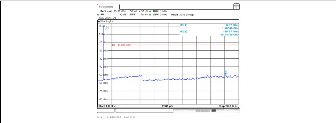
Band66-1.4MHz-16QAM-132665-1RB#0-Range4:1000~20000MHZ
