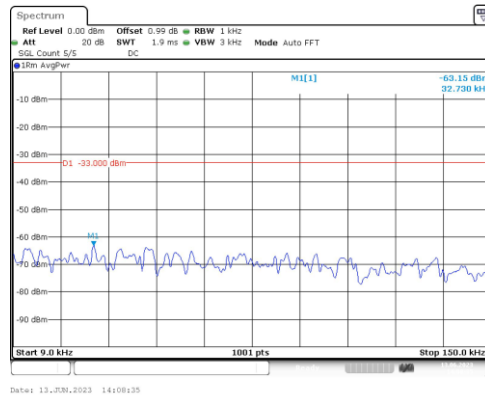
Band66-1.4MHz-QPSK-132665-1RB#0-Range1:0.009~0.15MHz
