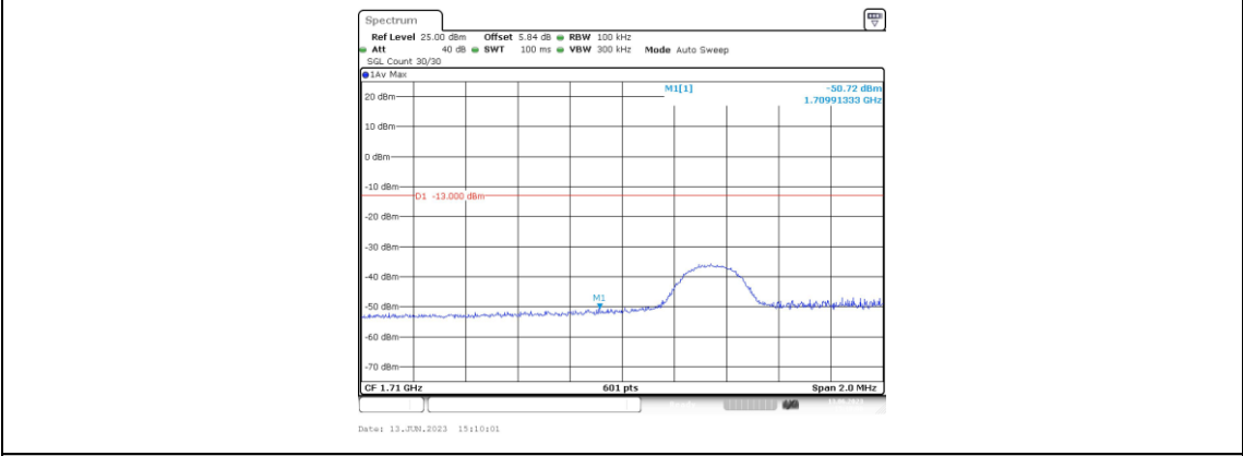
Band66-5MHz-QPSK-131997-1RB#24
