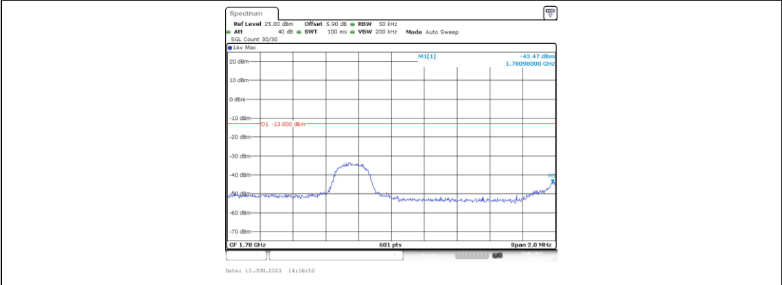
Band66-3MHz-QPSK-132657-1RB#0
