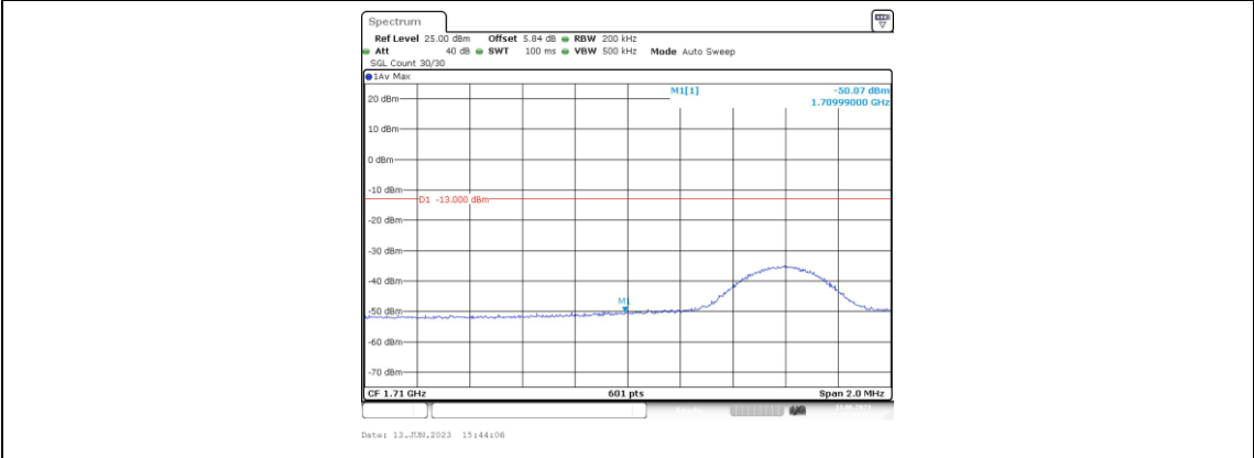
Band66-10MHz-16QAM-132022-1RB#49
