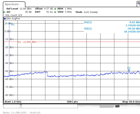
Band66-3MHz-16QAM-132322-1RB#0-Range4:1000~20000MHz
