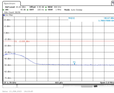
Band66-15MHz-QPSK-132597-1RB#0
