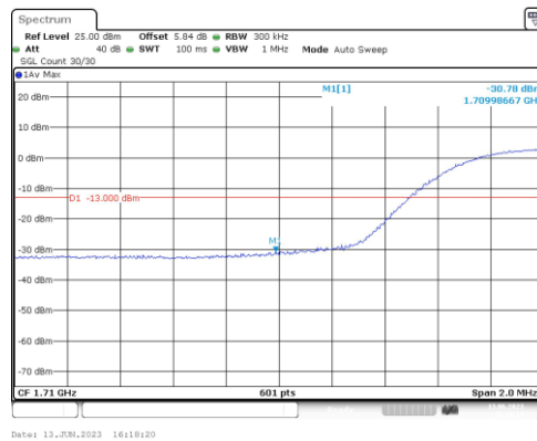
Band66-15MHz-16QAM-132047-75RB#0
