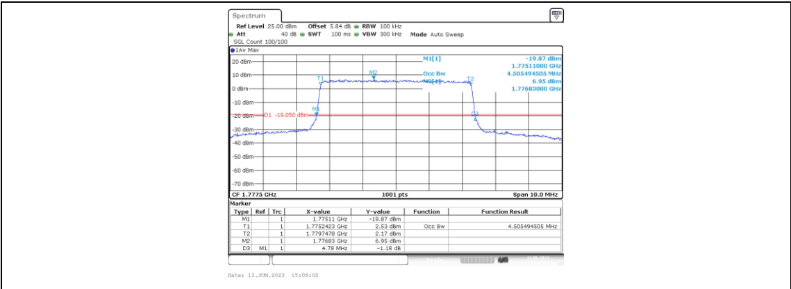
Band66-5MHz-16QAM-132647-25RB#0-4.505
