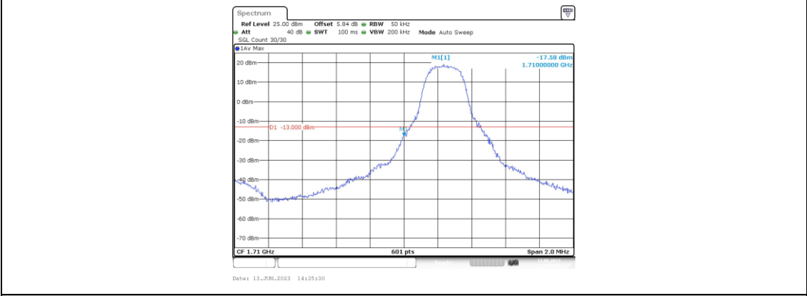
Band66-3MHz-QPSK-131987-1RB#0
