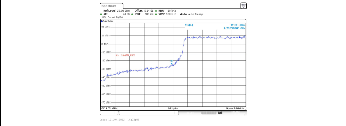
Band66-1.4MHz-QPSK-131979-6RB#0
