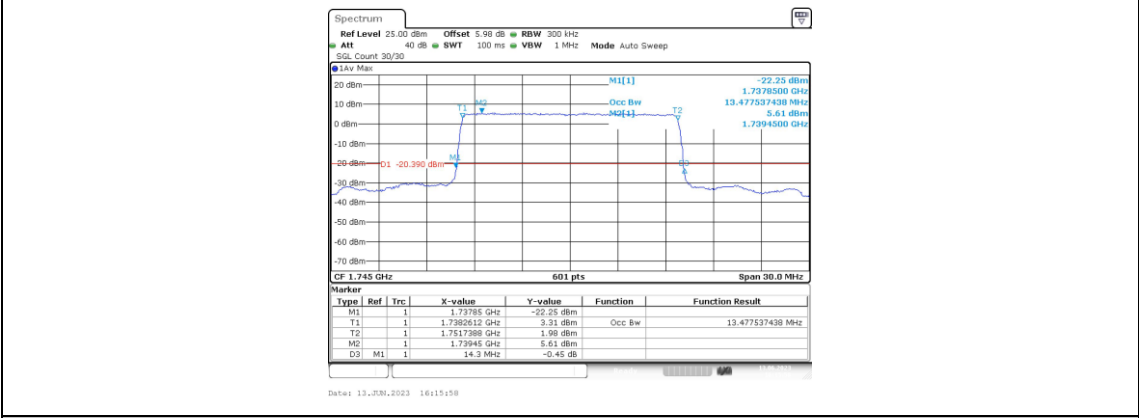
Band66-15MHz-QPSK-132322-75RB#0-13.478
