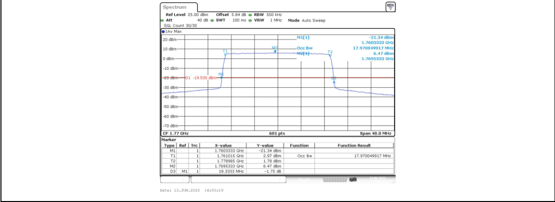
Band66-20MHz-16QAM-132322-100RB#0-18.037
