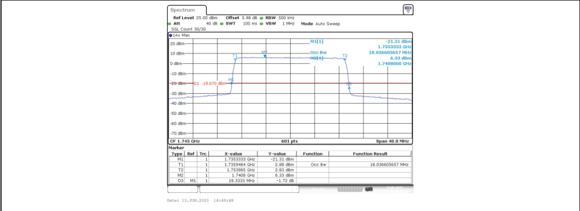
Band66-20MHz-QPSK-132322-100RB#0-18.037
