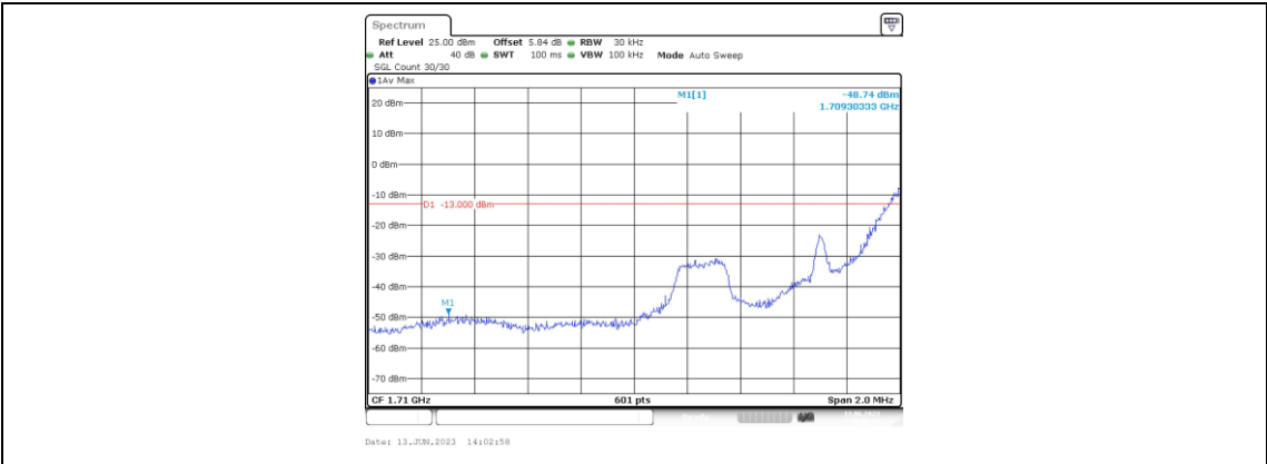
Band66-1.4MHz-16QAM-131979-1RB#5
