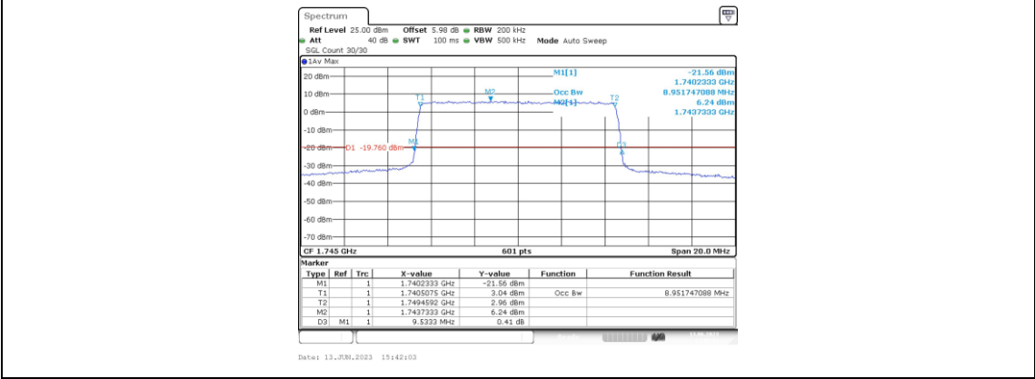
Band66-10MHz-16QAM-132022-50RB#0-8.952
