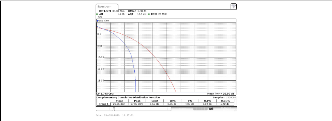
Band66-15MHz-QPSK-132322-1RB#0
