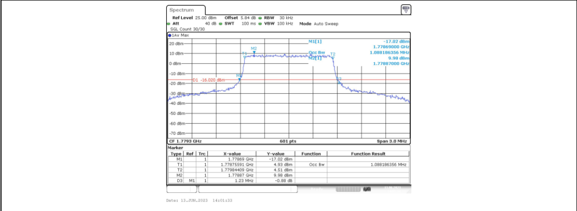
Band66-1.4MHz-QPSK-132665-6RB#0-1.088
