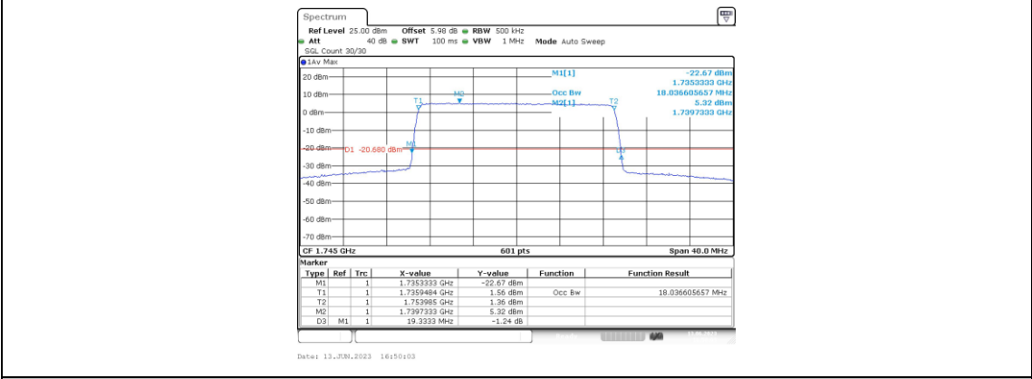
Band66-20MHz-16QAM-132322-100RB#0-18.037
