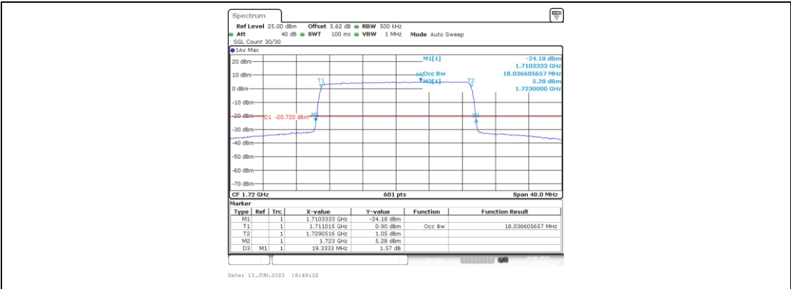
Band66-20MHz-16QAM-132072-100RB#0-18.037
