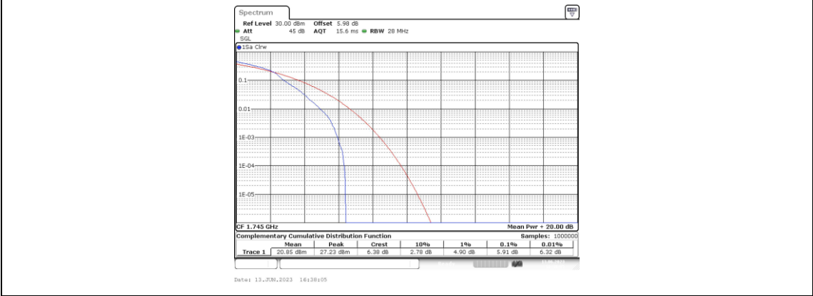
Band66-15MHz-16QAM-132322-1RB#0
