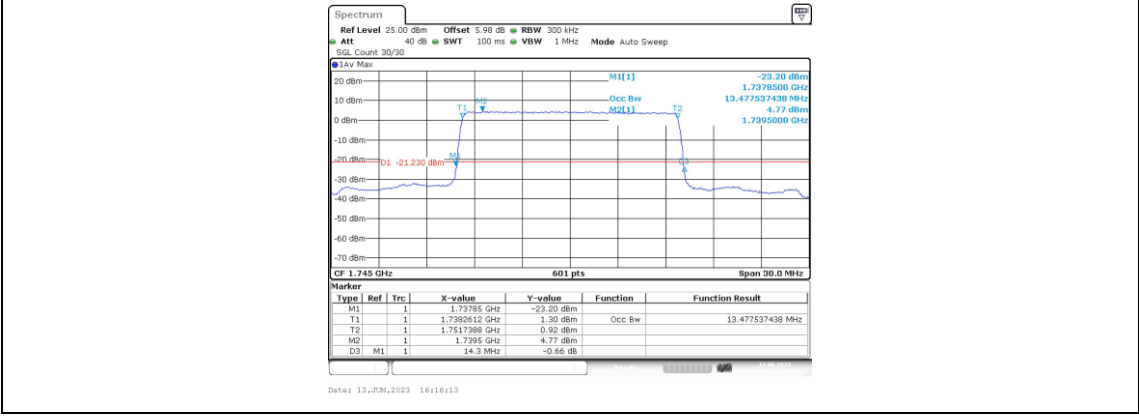
Band66-15MHz-QPSK-132322-75RB#0-13.478
