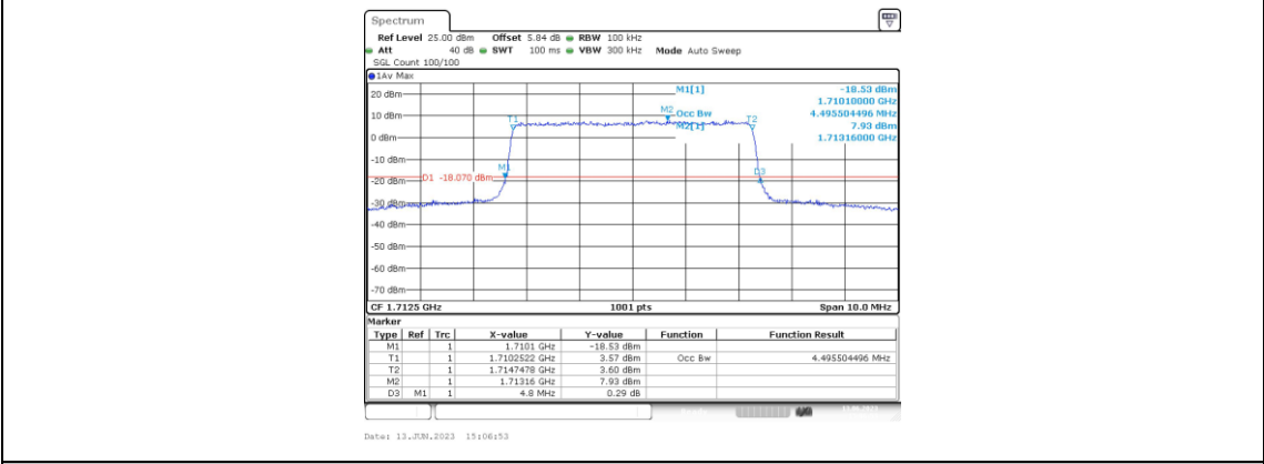
Band66-5MHz-QPSK-131997-25RB#0-4.496
