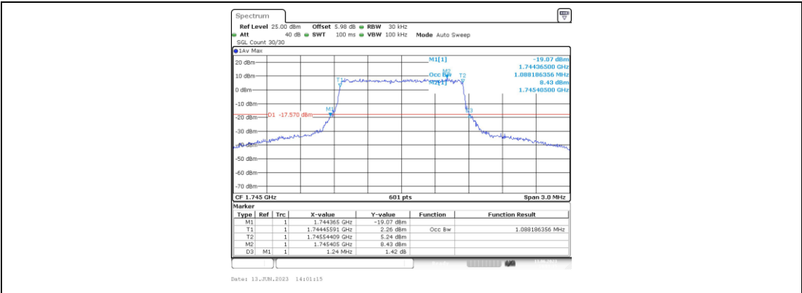
Band66-1.4MHz-16QAM-132322-6RB#0-1.088
