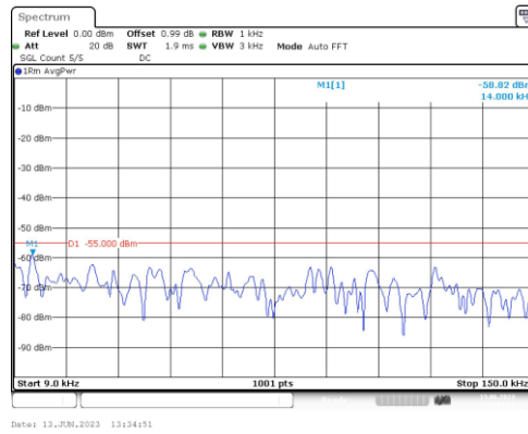
Band41-20MHz-16QAM-41490-1RB#0-Range1:0.009~0.15MHz
