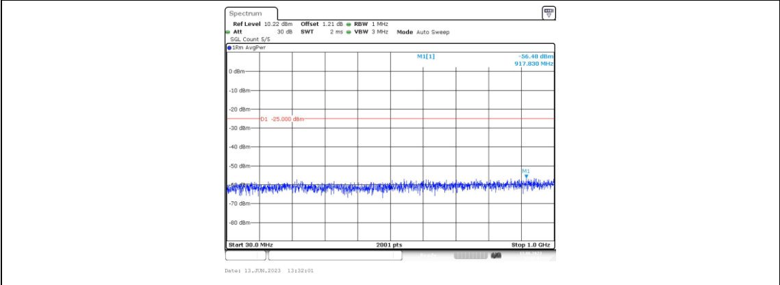
Band41-20MHz-QPSK-40620-1RB#0-Range3:30~1000MHz
