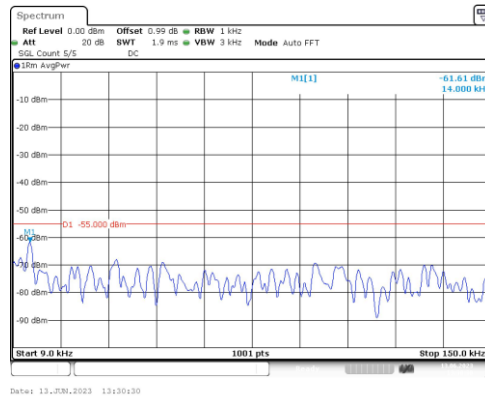
Band41-20MHz-16QAM-39750-1RB#0-Range1:0.009~0.15MHz
