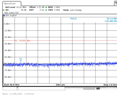
Band41-20MHz-16QAM-41490-1RB#0-Range3:30~1000MHz
