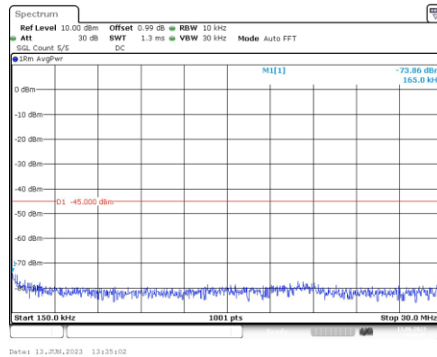
Band41-20MHz-16QAM-41490-1RB#0-Range2:0.15~30MHz
