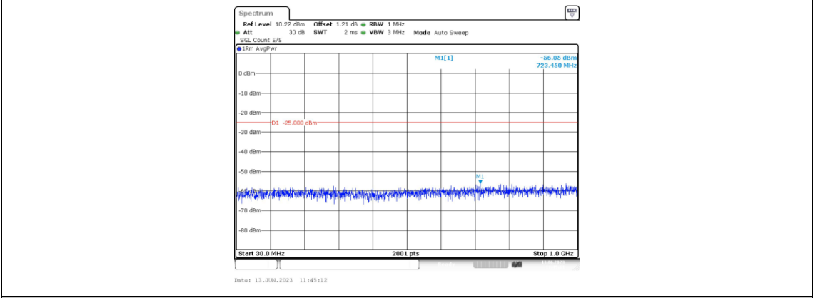
Band41-5MHz-QPSK-40620-1RB#0-Range3:30~1000MHz
