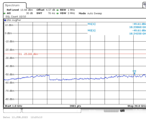
Band41-10MHz-16QAM-39700-1RB#0-Range4:1000~20000MHz
