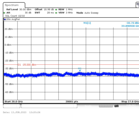
Band41-10MHz-16QAM-39700-1RB#0-Range5:20000~27000MHz
