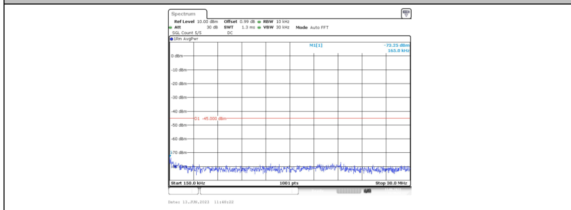
Band41-5MHz-16QAM-41565-1RB#0-Range2:0.15~30MHz
