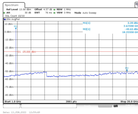
Band41-15MHz-16QAM-41515-1RB#0-Range4:1000~20000MHz
