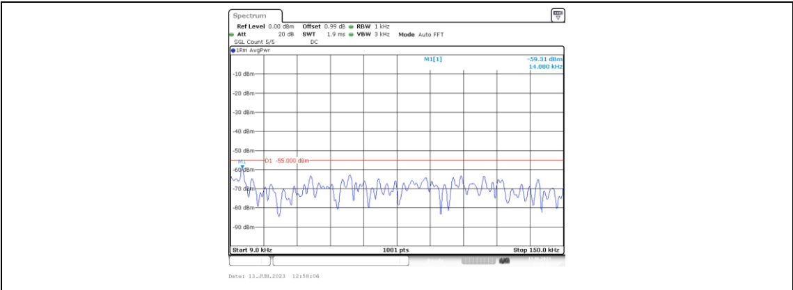
Band41-15MHz-QPSK-41515-1RB#0-Range1:0.009~0.15MHz
