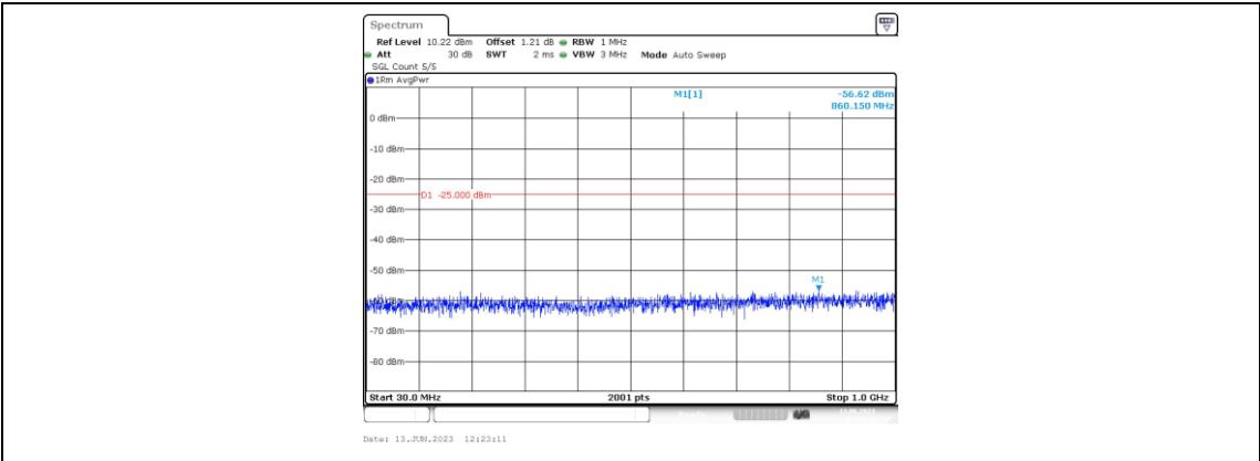
Band41-10MHz-QPSK-41540-1RB#0-Range3:30~1000MHz
