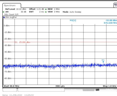
Band41-20MHz-QPSK-39750-1RB#0-Range3:30~1000MHz
