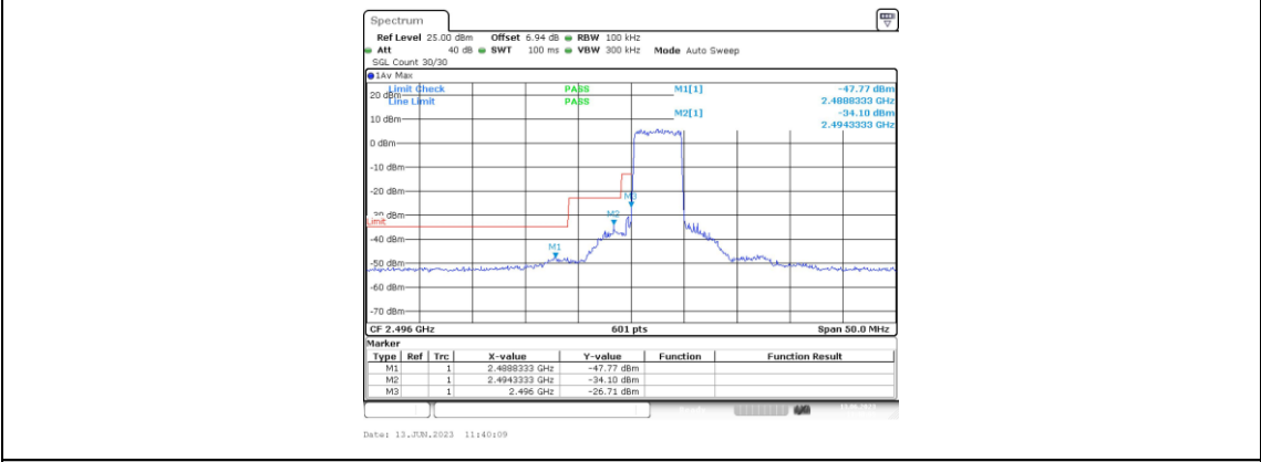
Band41-5MHz-QPSK-39675-25RB#0
