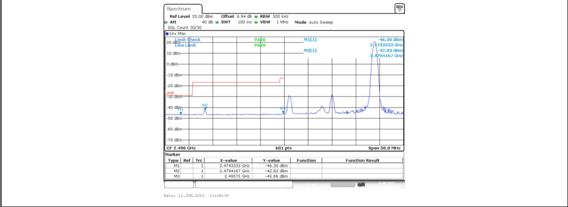
Band41-20MHz-QPSK-39750-1RB#99
