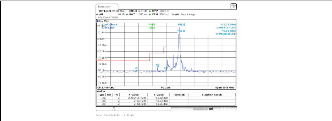
Band41-5MHz-QPSK-39675-1RB#24
