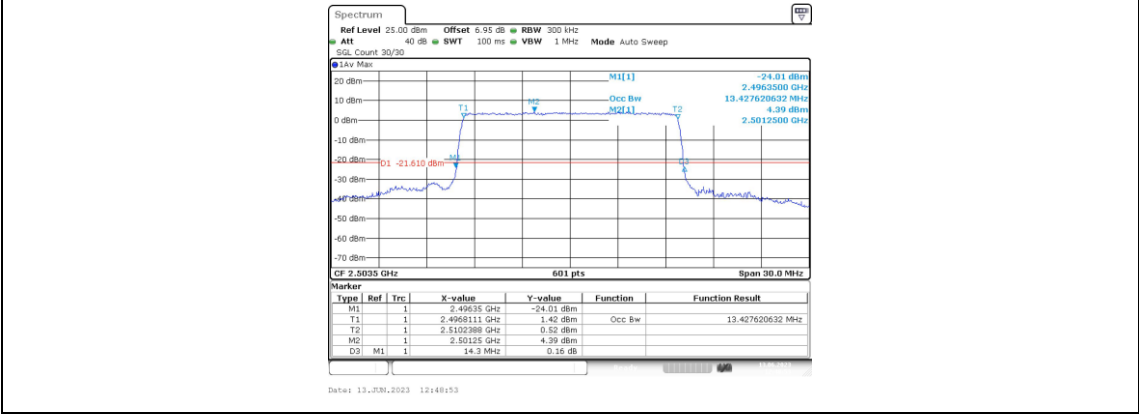
Band41-15MHz-QPSK-39725-75RB#0-13.478
