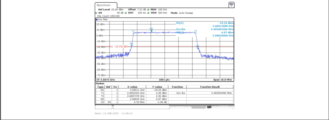
Band41-5MHz-QPSK-41565-25RB#0-4.496
