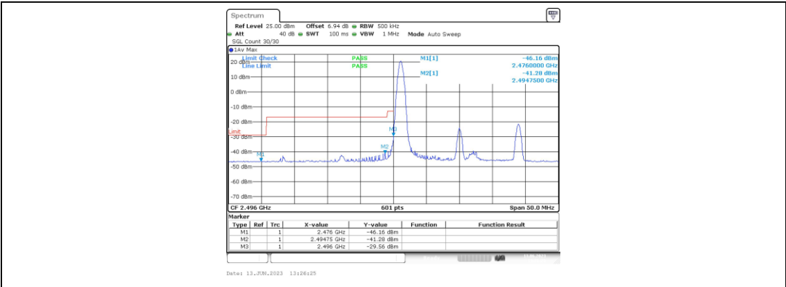
Band41-20MHz-16QAM-39750-1RB#0
